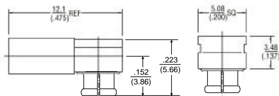
Right Angle Crimp Jack
