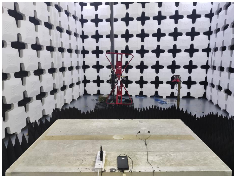
2. Radiated Emissions (Part 15B Camera/GSM receiver,1GHz-18GHz)
