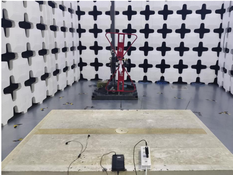
1. Radiated Emissions (Part 15B Camera/GSM receiver,30MHz-1GHz)
