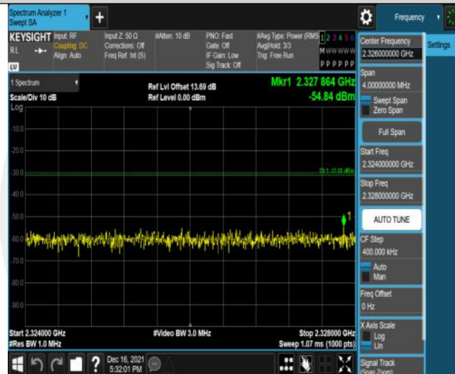
Band30-5MHz-QPSK-27685-25RB#0-Range8:2324~2328MHz
