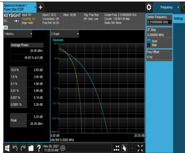
Band30-10MHz-QPSK-27710-50RB#0
