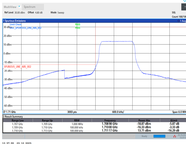
Band66-1.4MHz-QPSK-131979-6RB#0
