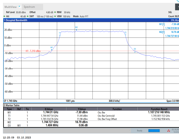
Band66-1.4MHz-16QAM-132322-6RB#0
