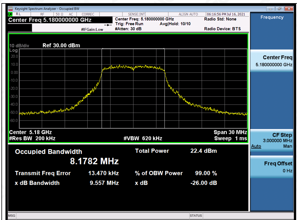
Test_Graph_OFDM_ANT2_5180_6Mbps_OBW
