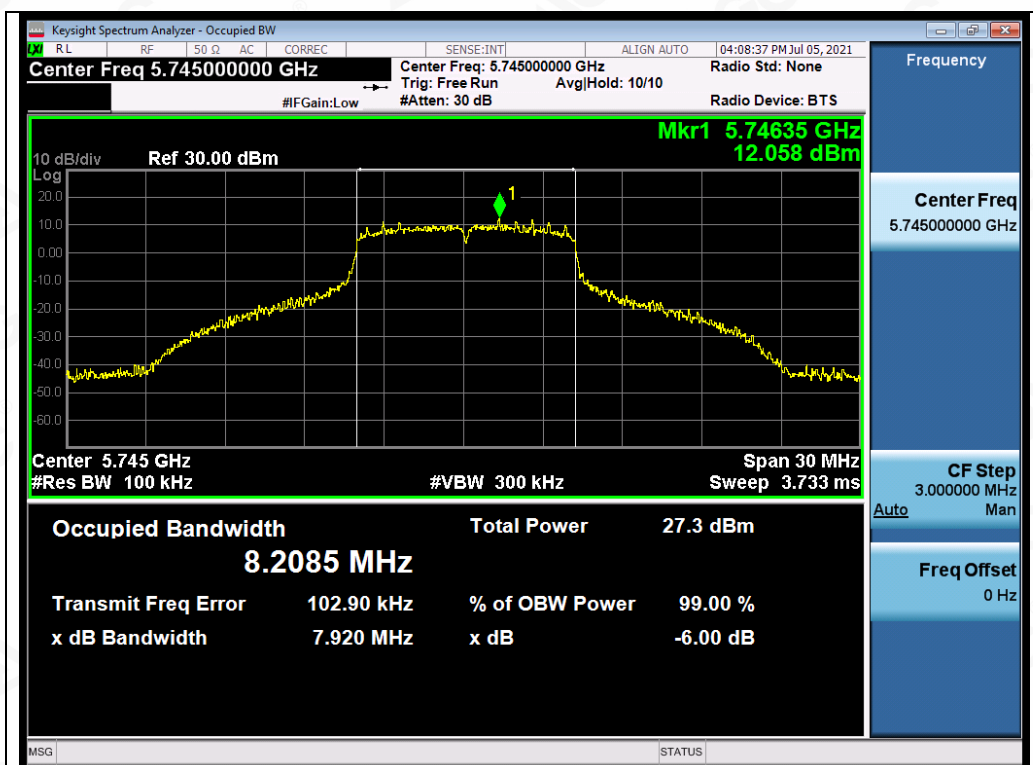
Test_Graph_OFDM_ANT2_5745_6Mbps_DTSBW
