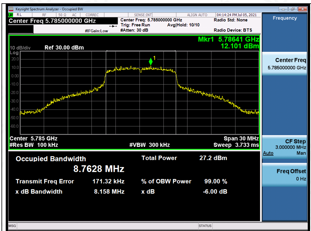
Test_Graph_OFDM_ANT2_5785_MCS0_DTSBW
