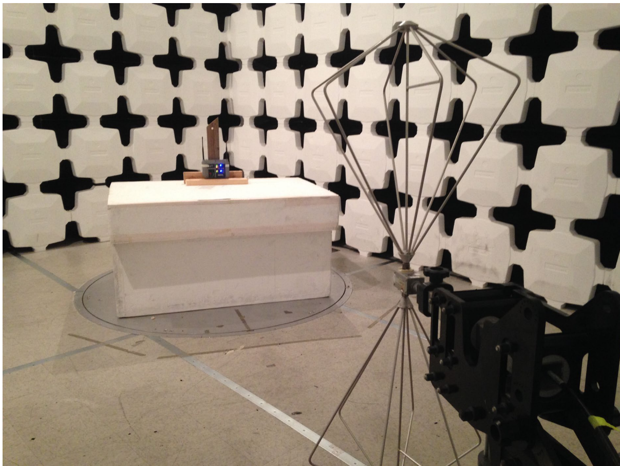
Figure 1. Radiated Emissions below 200 MHz
