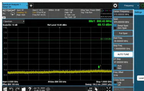
BLE_125K-Ant1-2440-30~1000-PASS
