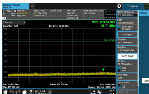
BLE_125K-Ant1-2480-30~1000-PASS
