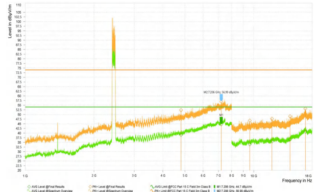
BLE_500K_2480_High
