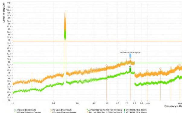
BLE_500K_2440_High
