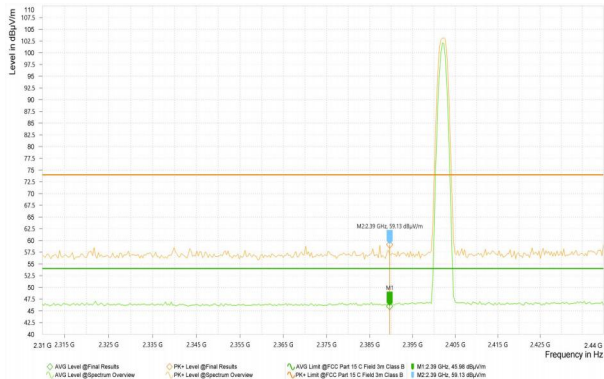
BLE_500K_2402
