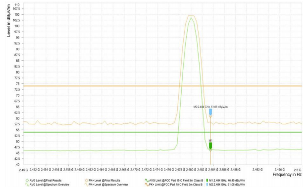
BLE_500K_2480
