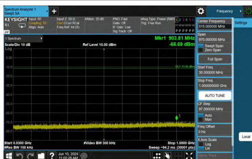
BLE_500K-Ant1-2480-30~1000-PASS
