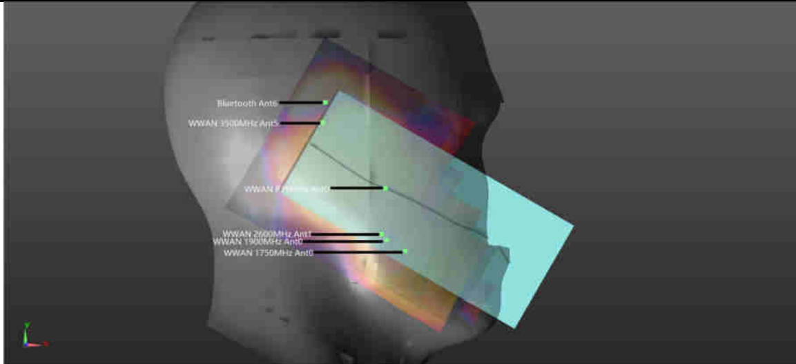
WWAN+FR1+BT Left Tilted
