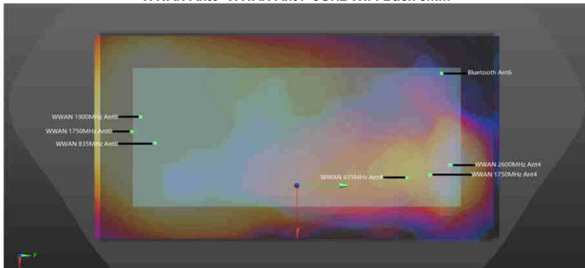
WWAN Ant0+WWAN Ant4+BT Back 5mm
