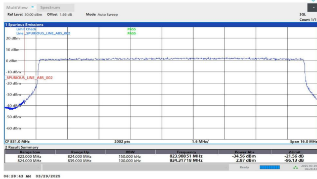
Band26(824-849)-15MHz-QPSK-26865-75RB#0-PASS
