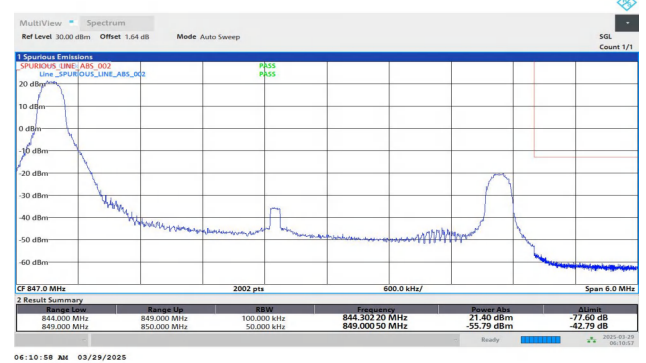
Band26(824-849)-5MHz-QPSK-27015-1RB#0-PASS
