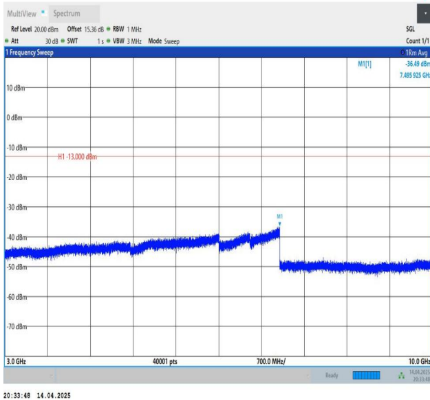
Band26(824-849)-1.4MHz-QPSK-26915-1RB#0-3000~10000-PASS
