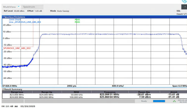
Band26(824-849)-5MHz-QPSK-26815-25RB#0-PASS
