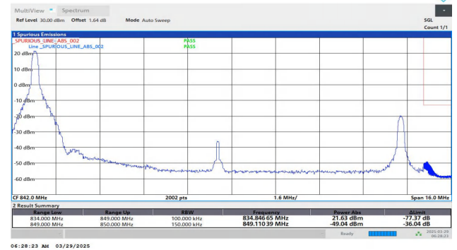
Band26(824-849)-15MHz-QPSK-26965-1RB#0-PASS
