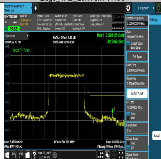
NTNV-N77-3450-3550-PC2-30-50-H-DFT-QPSK-Outer Full-
