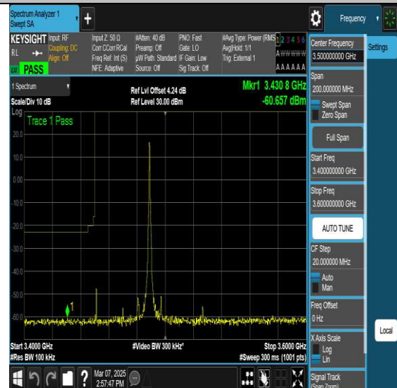
NTNV-N77-3450-3550-PC2-30-30-H-DFT-QPSK-Outer_Full-Ant1-PASS
