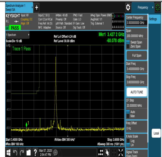
NTNV-N77-3450-3550-PC2-30-30-L-DFT-QPSK-
