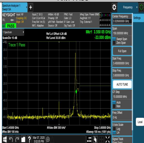
NTNV-N77-3450-3550-PC2-30-50-H-DFT-QPSK-
