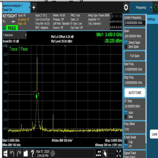
NTNV-N77-3450-3550-PC2-30-30-L-DFT-QPSK-
