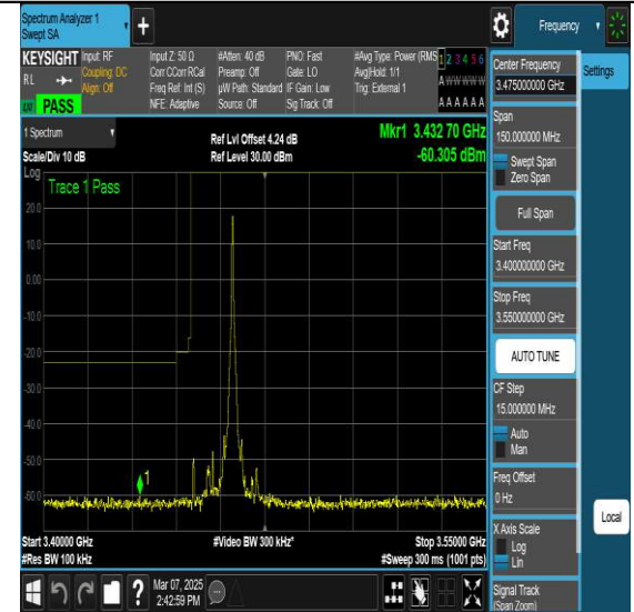
NTNV-N77-3450-3550-PC2-30-15-L-DFT-QPSK-Edge 1RB Right-Ant1-PASS
