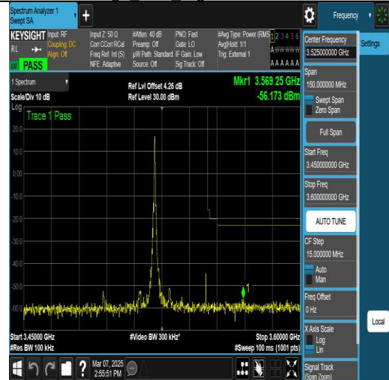
NTNV-N77-3450-3550-PC2-30-30-H-DFT-QPSK- Edge 1RB Left-Ant1-PASS
