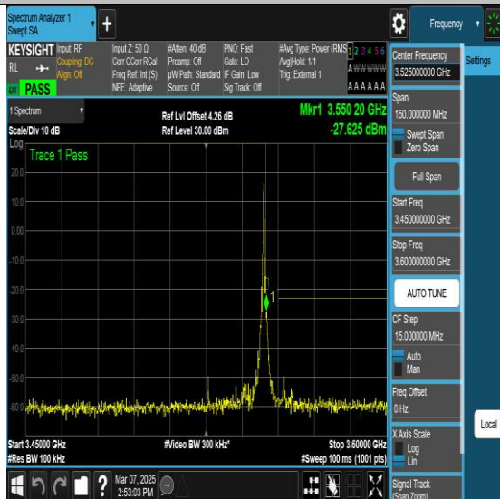
NTNV-N77-3450-3550-PC2-30-25-H-DFT-QPSK-Edge 1RB Right-Ant1-PASS
