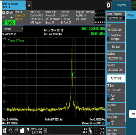
NTNV-N77-3450-3550-PC2-30-10-H-DFT-QPSK-Edge 1RB Right-Ant1-PASS
