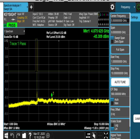
NTNV-N77-3450-3550-PC2-30-10-H-DFT-QPSK-
