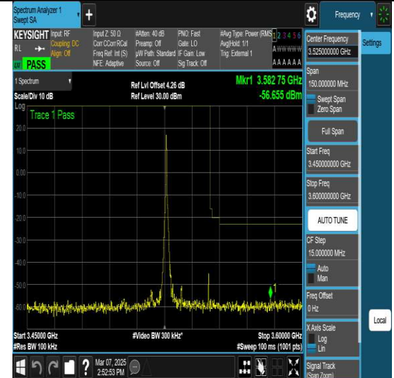
NTNV-N77-3450-3550-PC2-30-25-H-DFT-QPSK-Edge 1RB Left-Ant1-PASS
