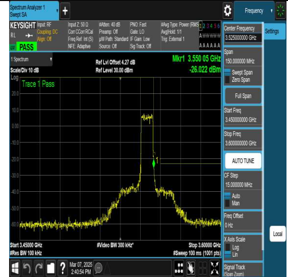
NTNV-N77-3450-3550-PC2-30-10-H-DFT-QPSK-Outer_Full-Ant1-PASS
