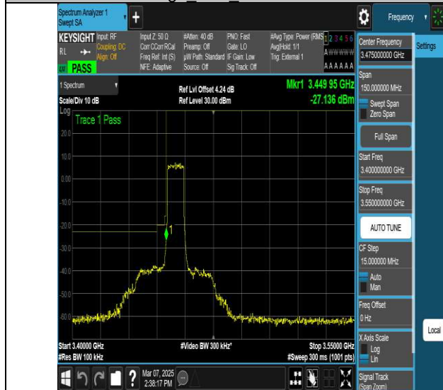
NTV-N77-3450-3550-PC2-30-10-L-DFT-QPSK-Outer_Full- Ant1-PASS
