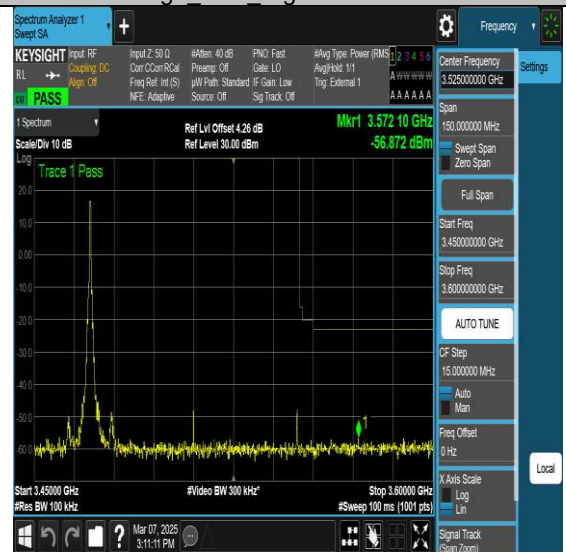
NTNV-N77-3450-3550-PC2-30-80-H-DFT-QPSK
