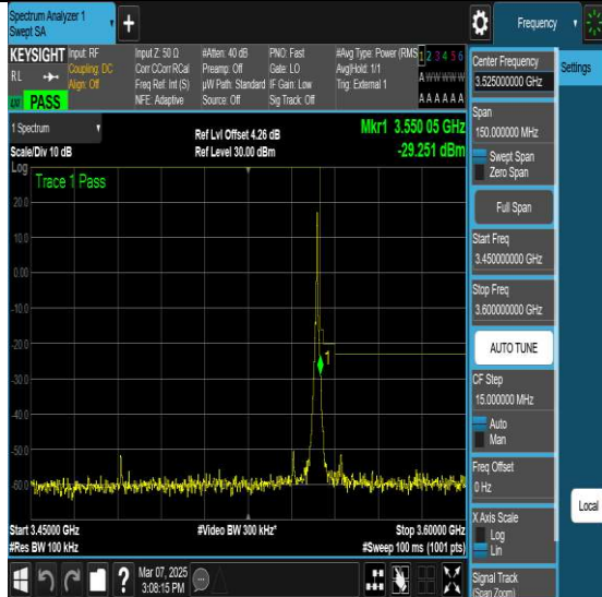
NTNV-N77-3450-3550-PC2-30-70-H-DFT-QPSK-Edge 1RB Right-Ant1-PASS
