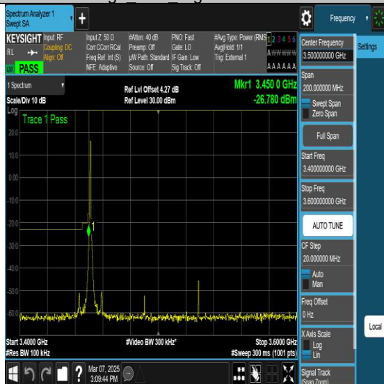
NTNV-N77-3450-3550-PC2-30-80-L-DFT-QPSK-Edge 1RB Left-Ant1-PASS
