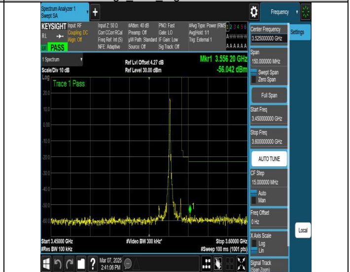
NTV-N77-3450-3550-PC2-30-10-H-DFT-QPSK- Edge 1RB Left-Ant1-PASS
