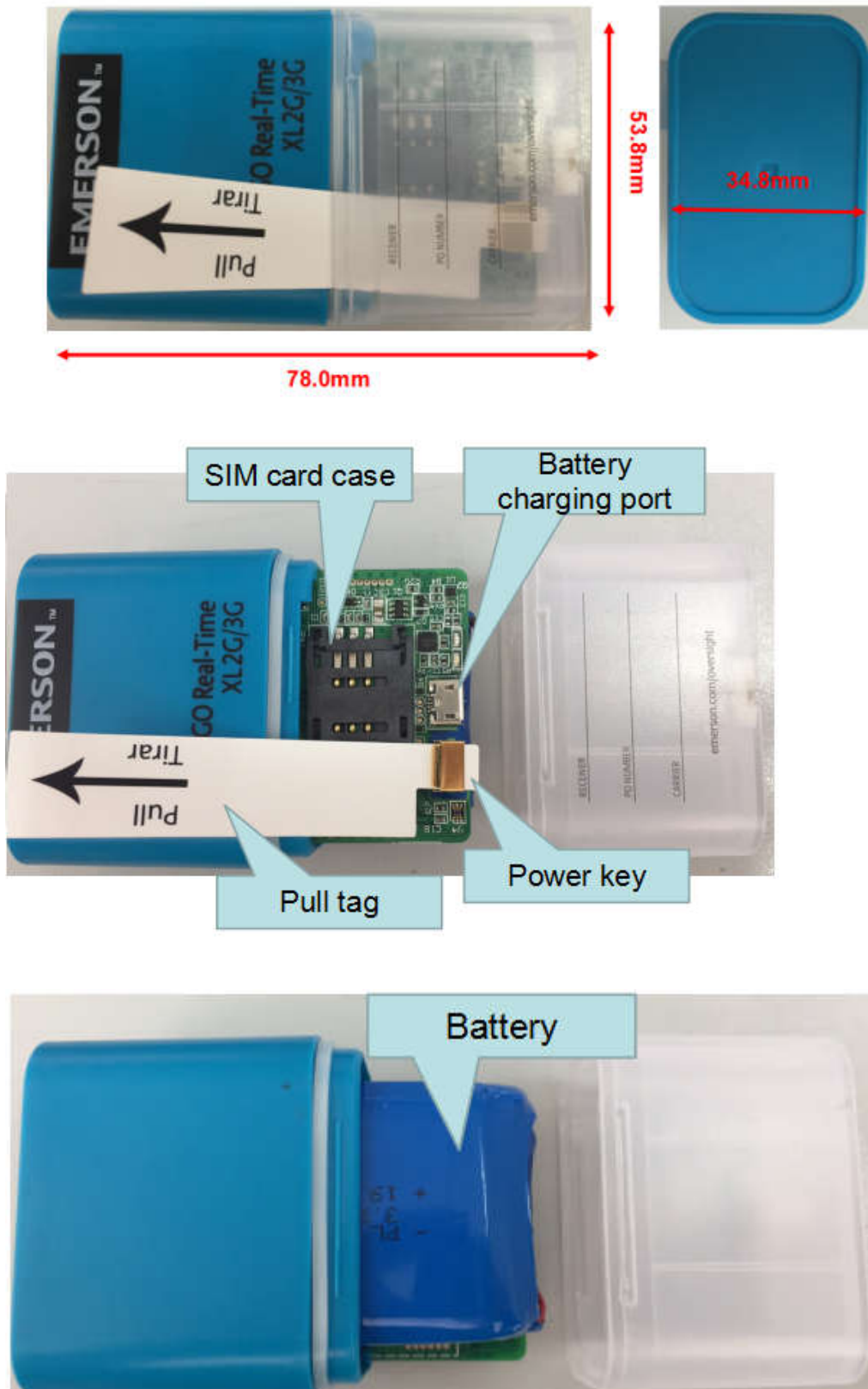
Figure 1 GO Real-Time 2G/3G Physical Attributes
