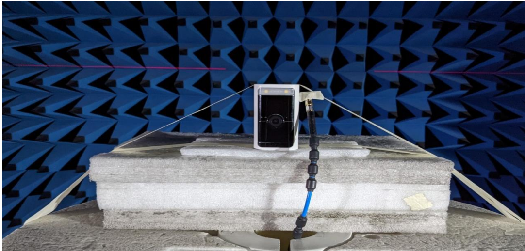
Setup Photo
