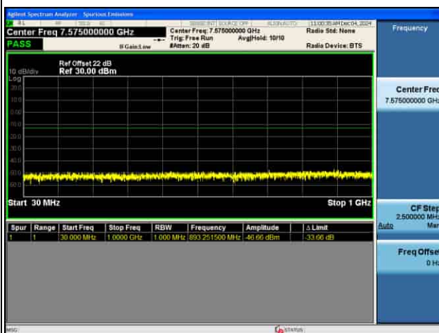
CSE_5G_n77(N)_30KHz_.PI2-BPSK_20M CH664666_1RB@1
