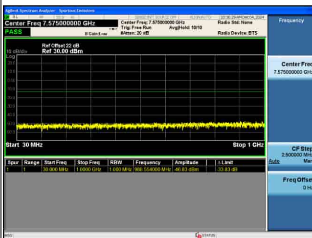
CSE_5G_n77(N)_30KHz_.PI2-BPSK_15M CH664832_1RB@1
