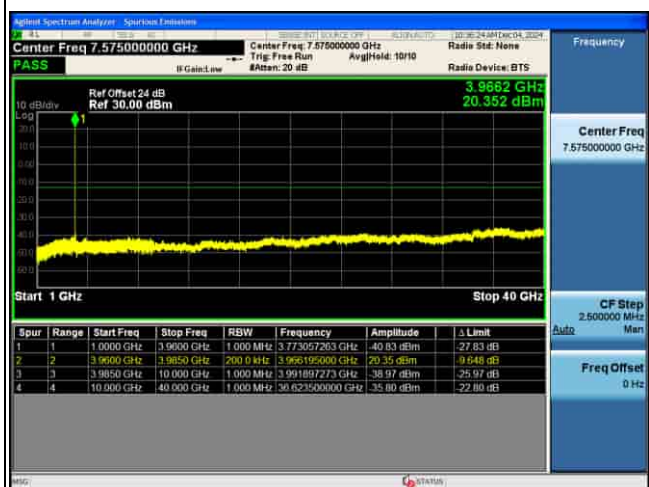
CSE_5G_n77(N)_30KHz_.PI2-BPSK_15M CH664832_1RB@1_
