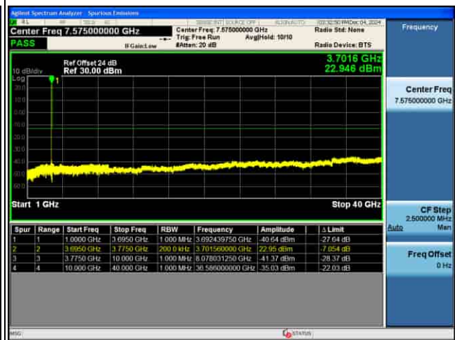
CSE_5G_n77(N)_30KHz_16QAM_70M CH656000_1RB@1_
