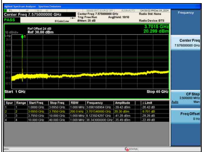
CSE_5G_n77(N)_30KHz_.PI2-BPSK_90M CH656000_1RB@1_
