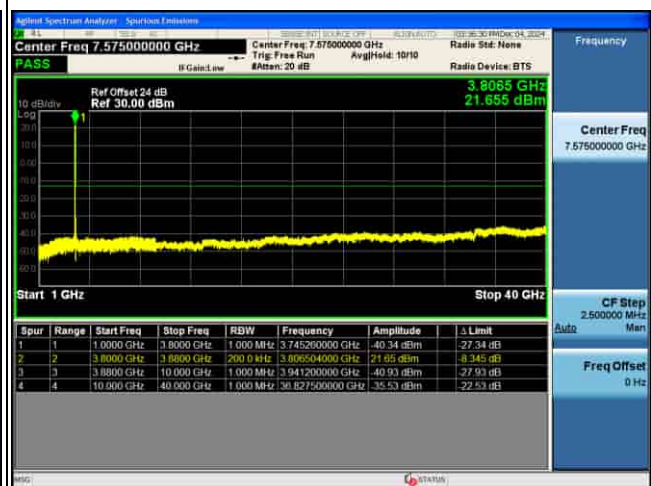
CSE_5G_n77(N)_30KHz_16QAM_70M CH663000_1RB@1_
