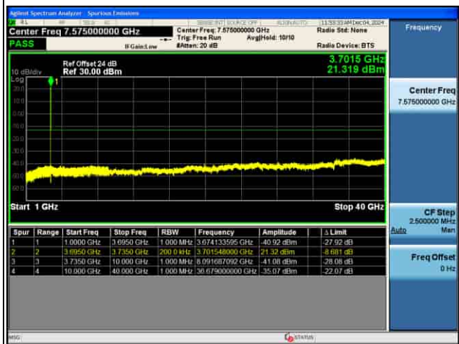
CSE_5G_n77(N)_30KHz_.PI2-BPSK_30M CH656000_1RB@1_
