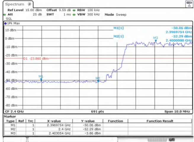
Out Of Band Emission(Left) \pi/4 QPSK_2-DH5_Channel Hopping
