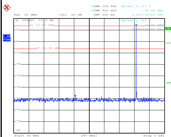
CSE Plot on CH 39 between 30 MHz ~ 3 GHz
