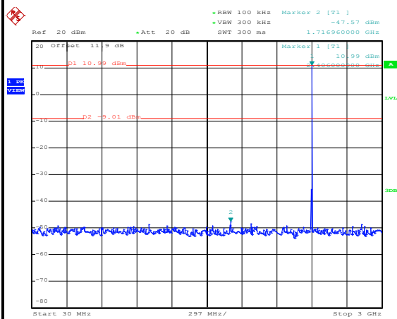
CSE Plot on CH 00 between 30 MHz ~ 3 GHz
