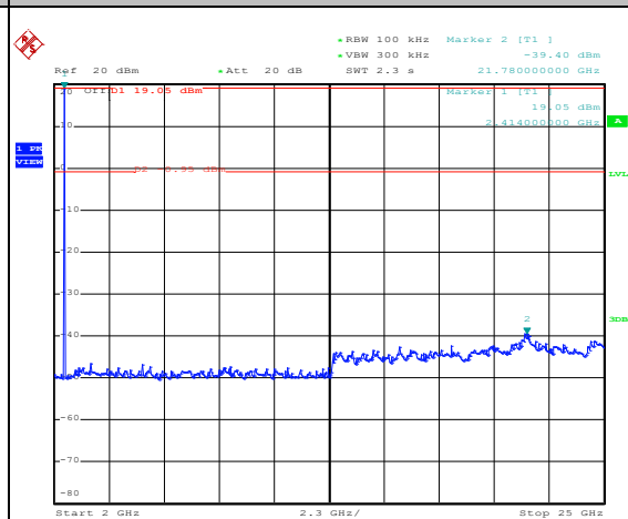
CSE Plot on CH 39 between 2 GHz ~ 25 GHz
