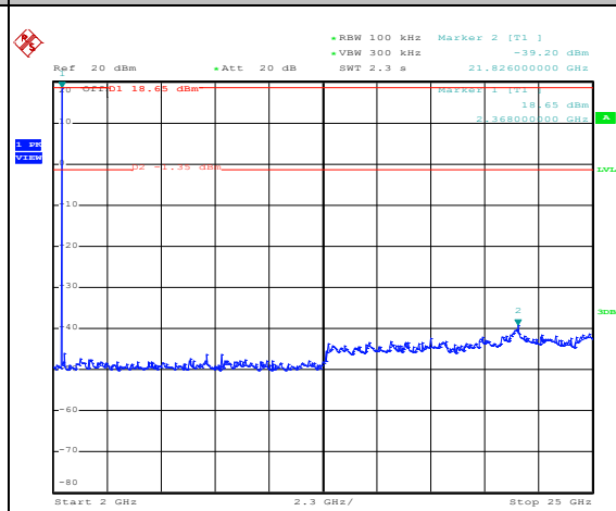
CSE Plot on CH 00 between 2 GHz ~ 25 GHz
