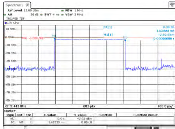
GFSK DH3
