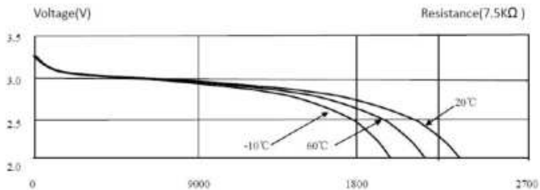
Discharge characteristic on load
