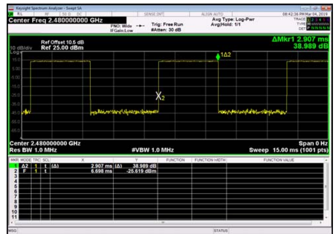
DQPSK,2480,2DH5,Transmission Time
