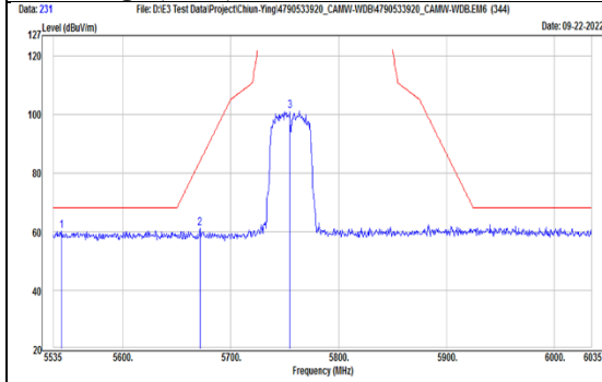
TX, 802.11ac(VHT40) (Ch 151) Band Edge (Peak), Horizontal
