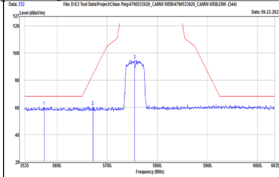
TX, 802.11ac(VHT40) (Ch 151) Band Edge (Peak), Vertical
