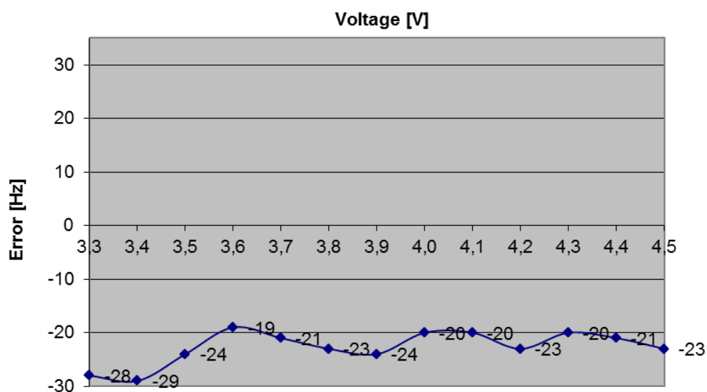
Channel 661 - E-GPRS Frequency error due to voltage variations
