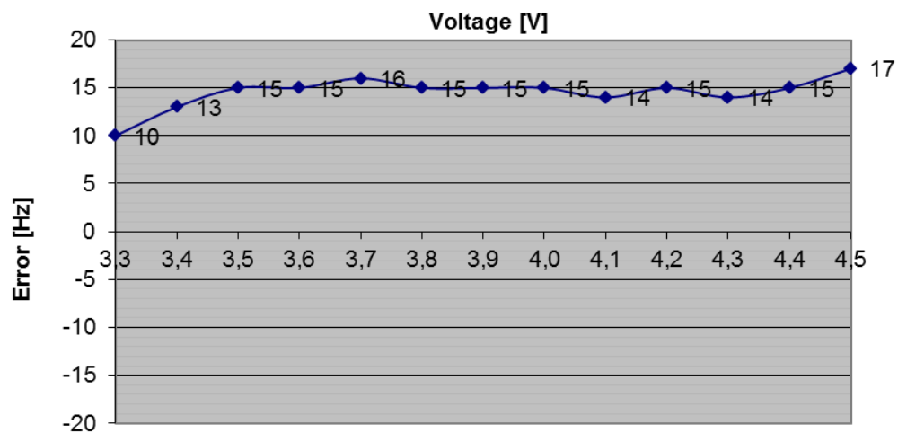
Channel 192 - GSM Frequency error due to voltage variations
