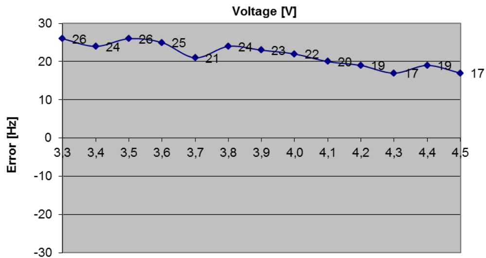
Channel 661- GSM Frequency error due to voltage variations
