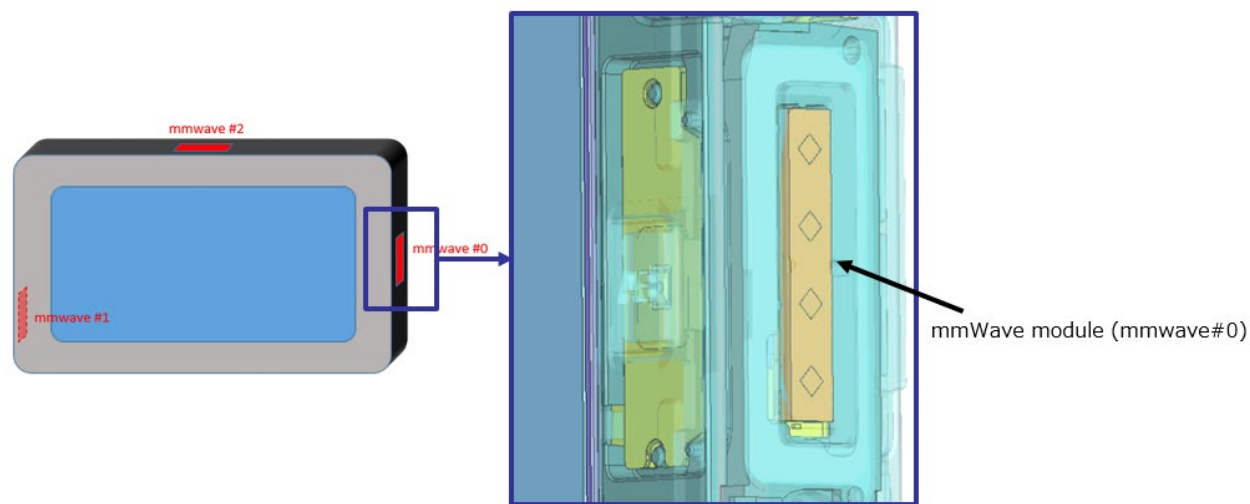
Figure 4. mmWave module
