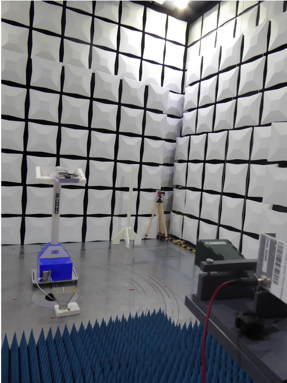
Test setup 18 – 26.5 GHz
