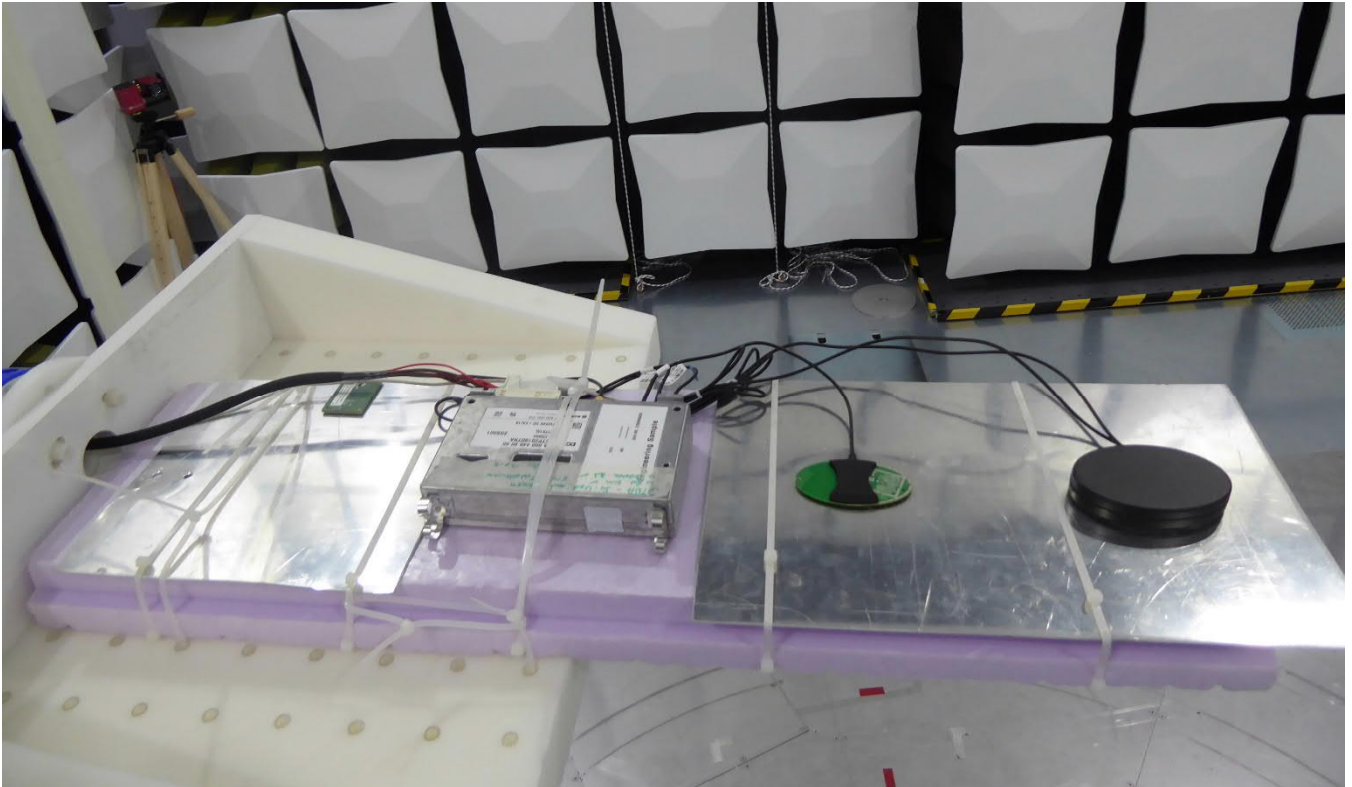
Test setup on positioner
