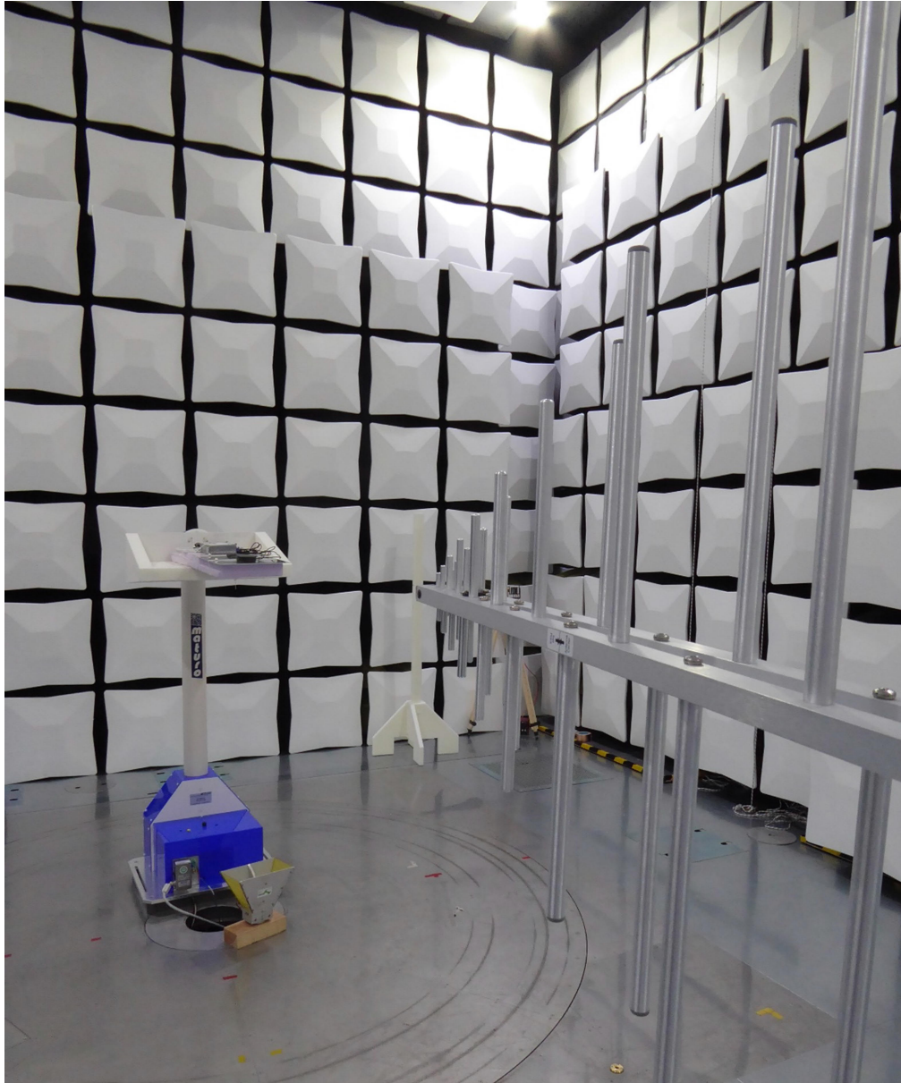
Test setup 200 MHz - 1 GHz
