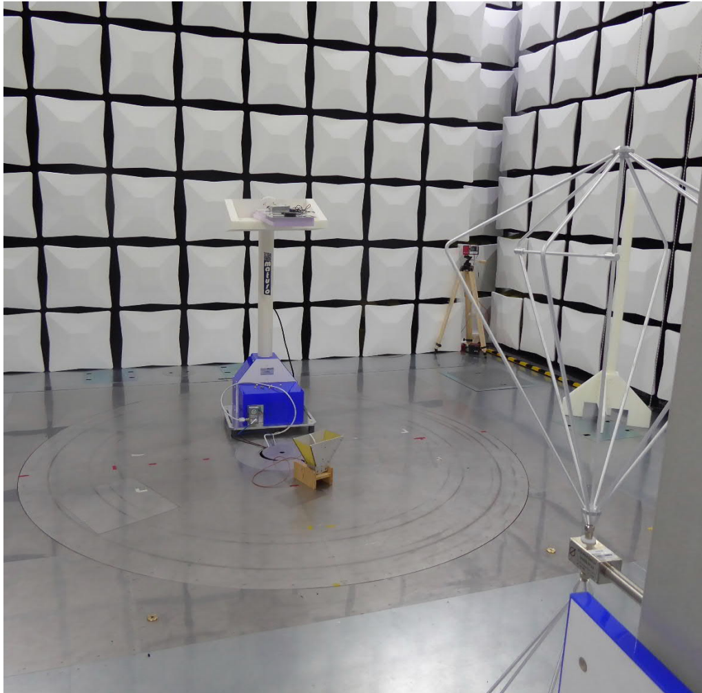
Test setup 30 - 200 MHz
