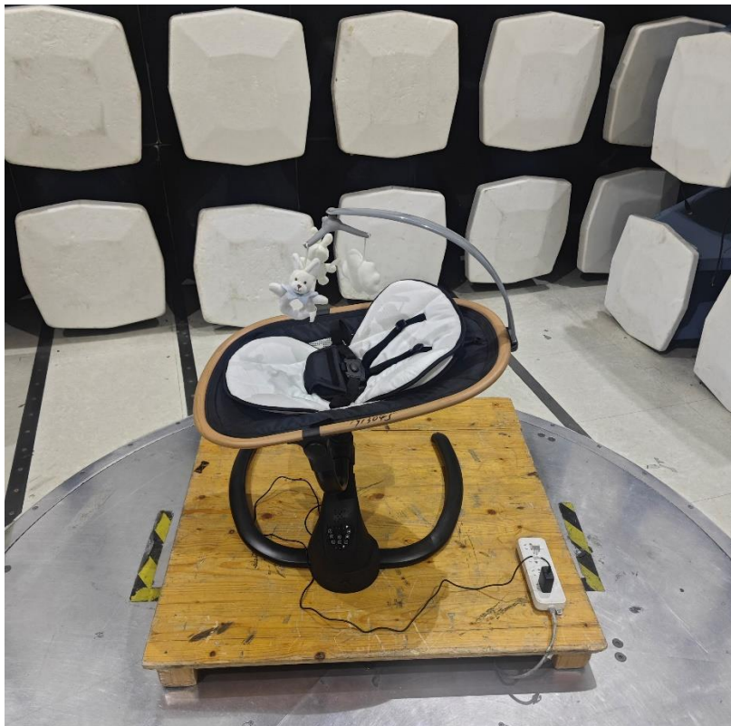
(The EUT placed at the center of the turntable)
