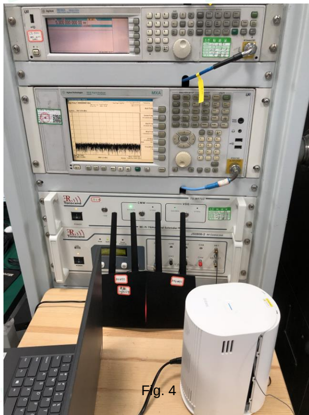
Test Setup Photo(s) of DFS Measurement
