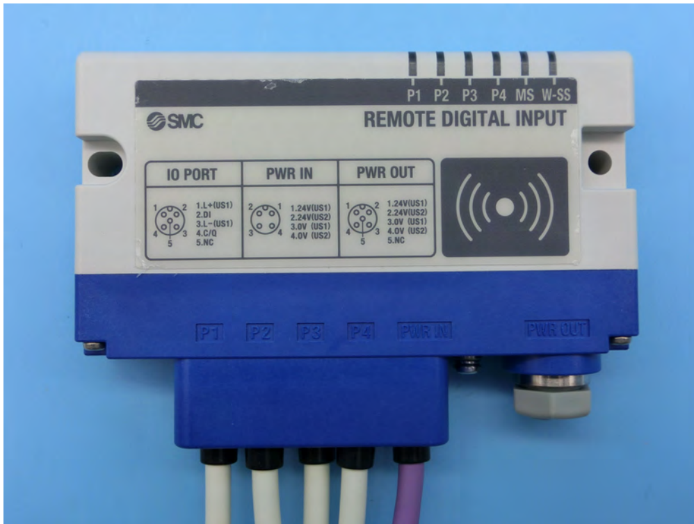
EX600-WLXB1 Front side
