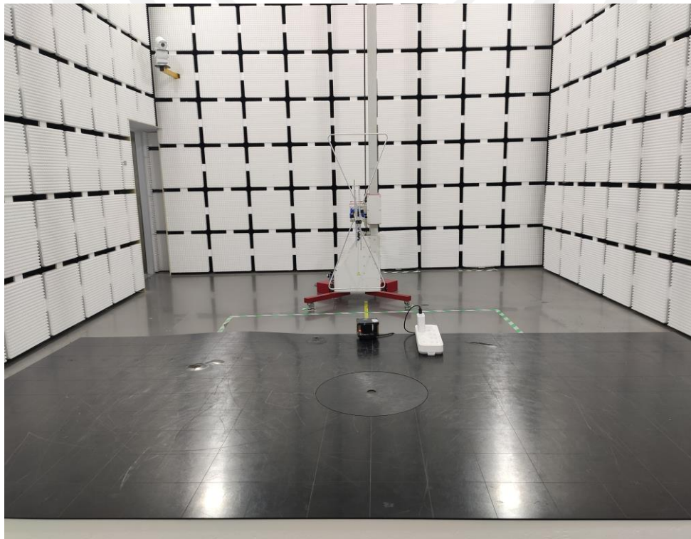
Spurious Radiation Emissions Test (<1G)
