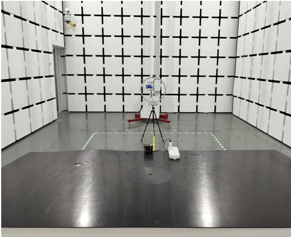
Spurious Radiation Emissions Test (<30M)
