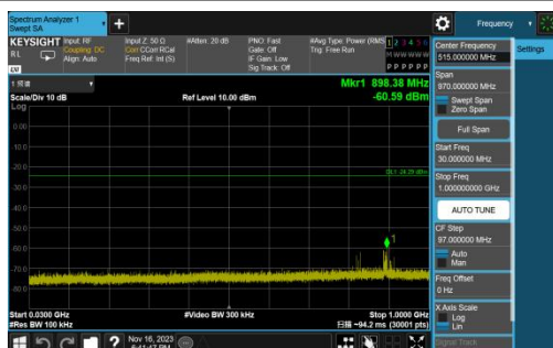
11B-Ant1-2412-30~1000-PASS
