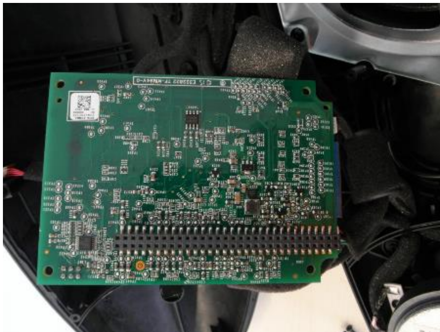
Photo 13: PCB 3 backside
