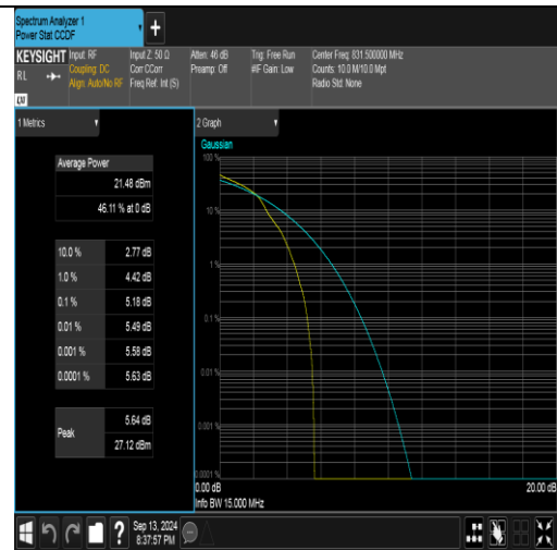
Band26(824-849)-15MHz-16QAM-26865-1RB#0-PASS
