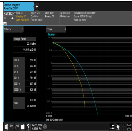
Band26(824-849)-1.4MHz-16QAM-26915-6RB#0-PASS
