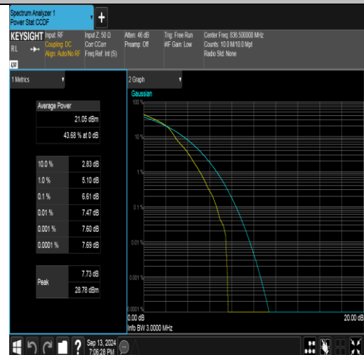
Band26(824-849)-3MHz-16QAM-26915-1RB#0-PASS
