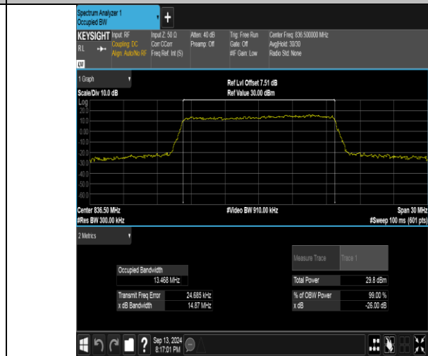
Band26(824-849)-15MHz-16QAM-26915-75RB#0-PASS
