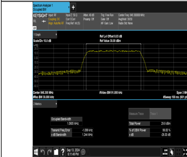
Band26(824-849)-1.4MHz-QPSK-27033-6RB#0-PASS
