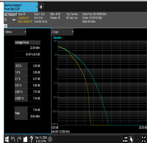
Band26(824-849)-10MHz-16QAM-26915-1RB#0-PASS
