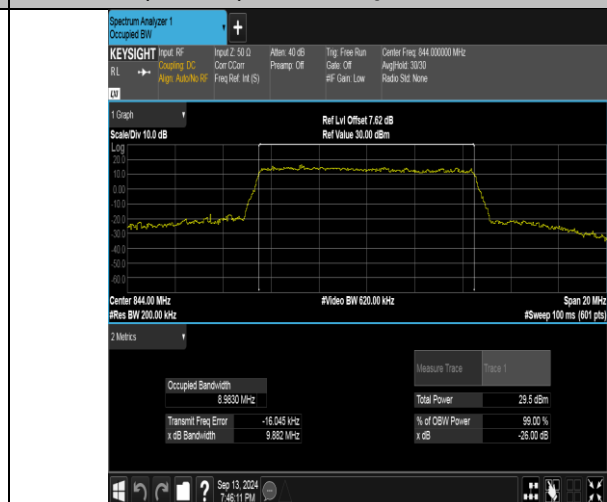
Band26(824-849)-10MHz-16QAM-26990-50RB#0-PASS
