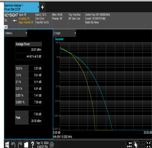
Band26(824-849)-15MHz-16QAM-26965-75RB#0-PASS
