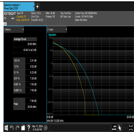
Band26(824-849)-10MHz-16QAM-26915-50RB#0-PASS
