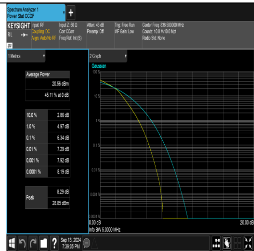
Band26(824-849)-5MHz-16QAM-26915-25RB#0-PASS
