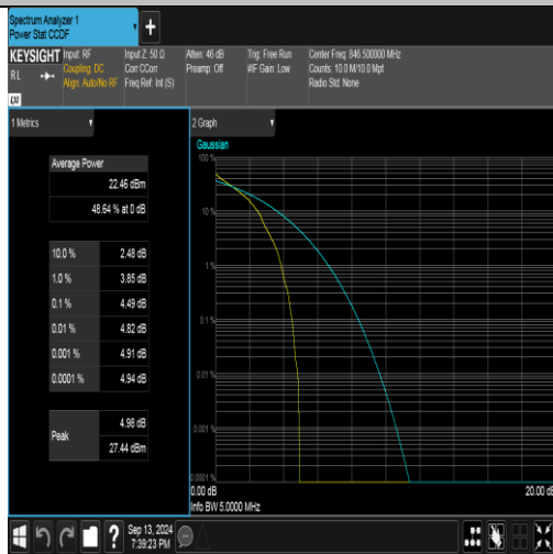
Band26(824-849)-5MHz-QPSK-27015-1RB#0-PASS
