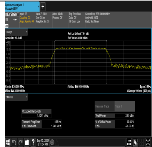
Band26(824-849)-1.4MHz-16QAM-26915-6RB#0-PASS
