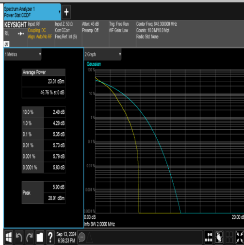
Band26(824-849)-1.4MHz-QPSK-27033-1RB#0-PASS
