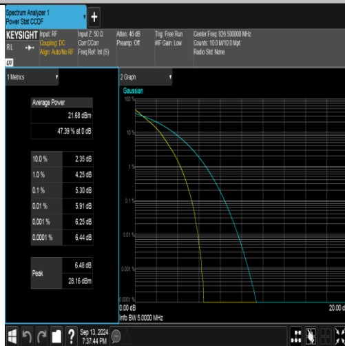
Band26(824-849)-5MHz-QPSK-26815-25RB#0-PASS
