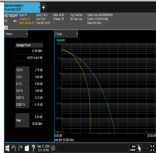
Band26(824-849)-10MHz-16QAM-26990-1RB#0-PASS
