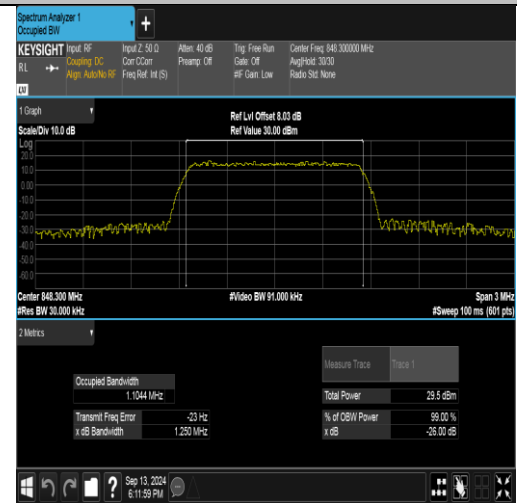
Band26(824-849)-1.4MHz-16QAM-27033-6RB#0-PASS
