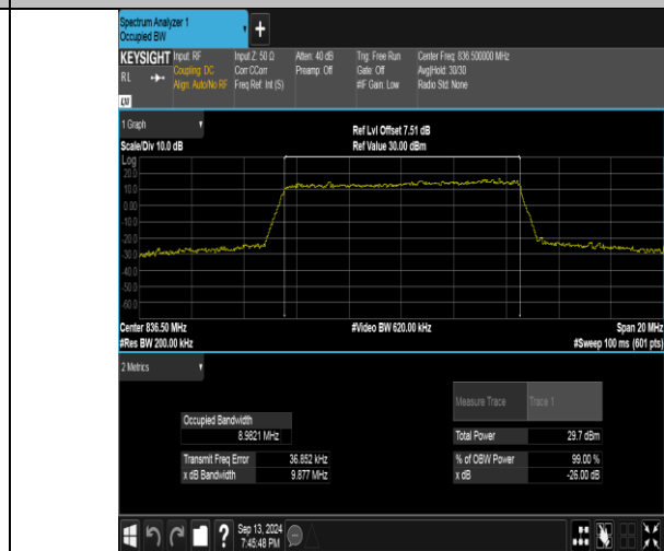
Band26(824-849)-10MHz-16QAM-26915-50RB#0-PASS
