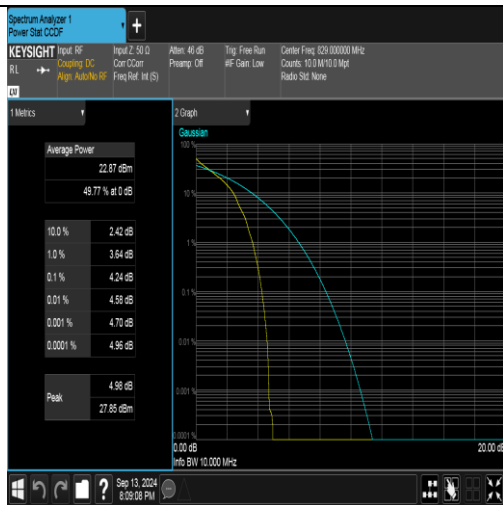
Band26(824-849)-10MHz-QPSK-26840-1RB#0-PASS
