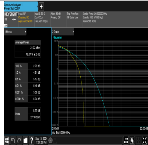
Band26(824-849)-5MHz-16QAM-26815-1RB#0-PASS
