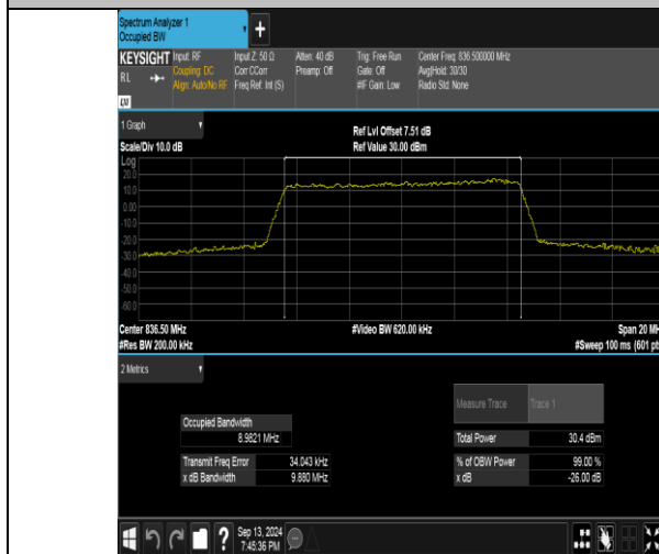
Band26(824-849)-10MHz-QPSK-26915-50RB#0-PASS
