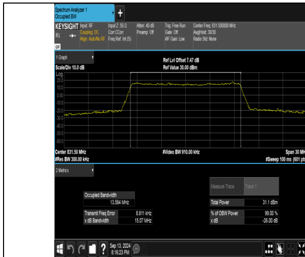
Band26(824-849)-15MHz-QPSK-26865-75RB#0-PASS
