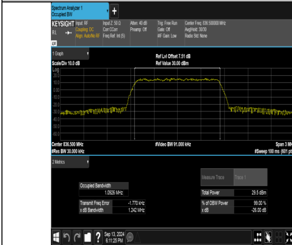
Band26(824-849)-1.4MHz-QPSK-26915-6RB#0-PASS
