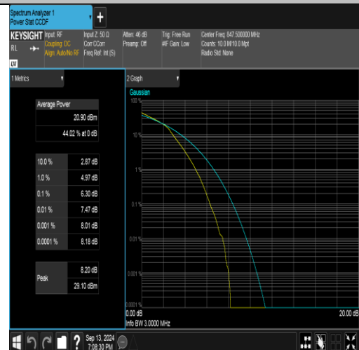
Band26(824-849)-3MHz-16QAM-27025-15RB#0-PASS
