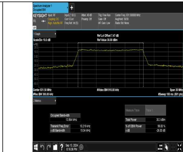
Band26(824-849)-15MHz-16QAM-26865-75RB#0-PASS
