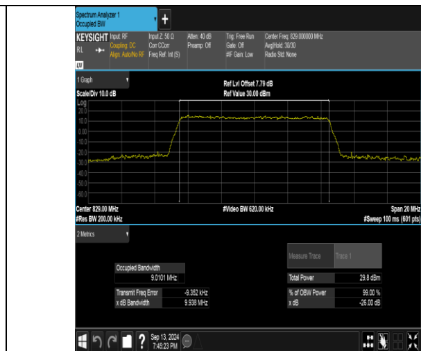
Band26(824-849)-10MHz-16QAM-26840-50RB#0-PASS
