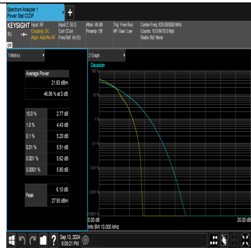
Band26(824-849)-10MHz-16QAM-26840-1RB#0-PASS
