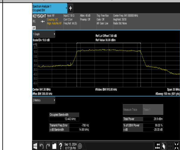
Band26(824-849)-15MHz-16QAM-26965-75RB#0-PASS
