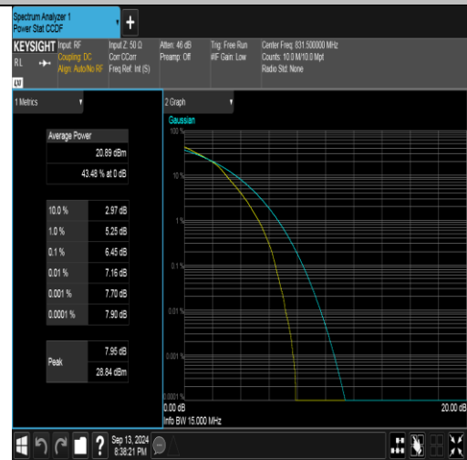
Band26(824-849)-15MHz-16QAM-26865-75RB#0-PASS
