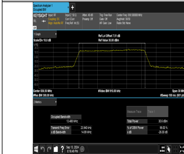
Band26(824-849)-15MHz-QPSK-26915-75RB#0-PASS
