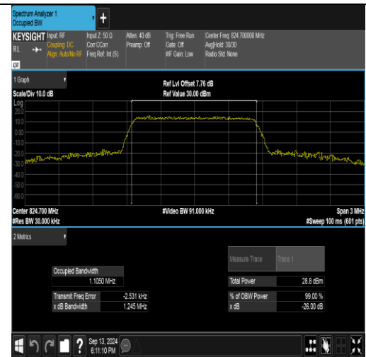
Band26(824-849)-1.4MHz-16QAM-26797-6RB#0-PASS
