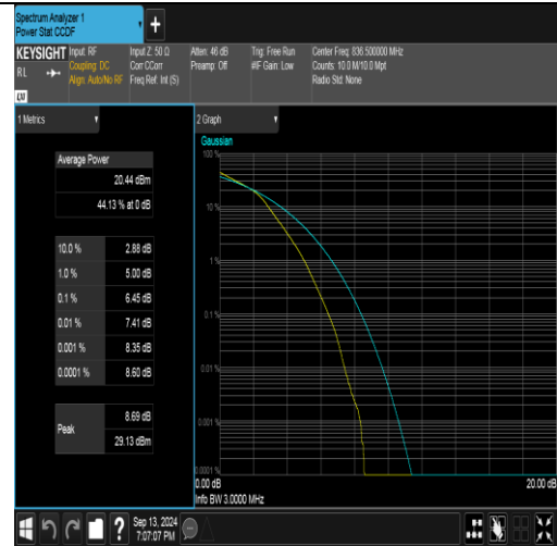
Band26(824-849)-3MHz-16QAM-26915-15RB#0-PASS
