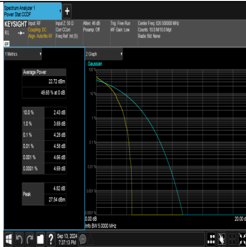
Band26(824-849)-5MHz-QPSK-26815-1RB#0-PASS
