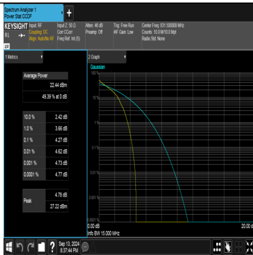
Band26(824-849)-15MHz-QPSK-26865-1RB#0-PASS
