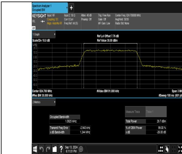
Band26(824-849)-1.4MHz-QPSK-26797-6RB#0-PASS
