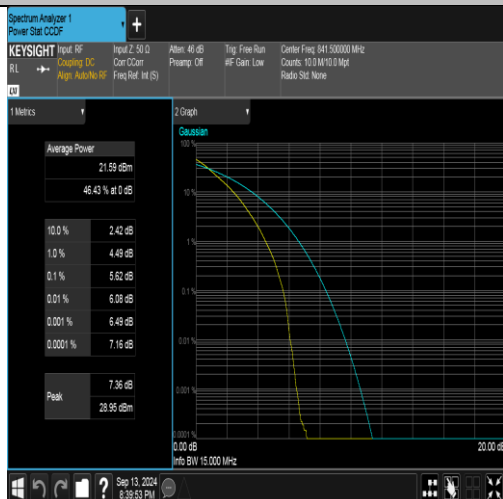
Band26(824-849)-15MHz-QPSK-26965-75RB#0-PASS
