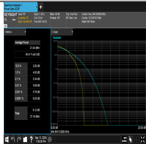
Band26(824-849)-5MHz-16QAM-27015-1RB#0-PASS
