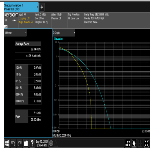
Band26(824-849)-1.4MHz-16QAM-27033-1RB#0-PASS
