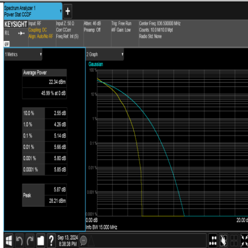
Band26(824-849)-15MHz-QPSK-26915-1RB#0-PASS
