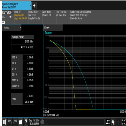
Band26(824-849)-15MHz-QPSK-26915-75RB#0-PASS
