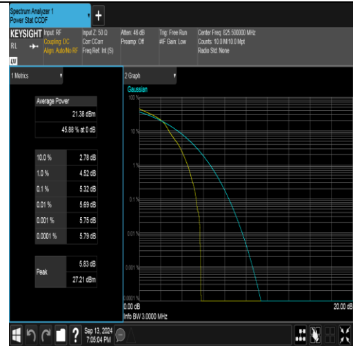
Band26(824-849)-3MHz-16QAM-26805-1RB#0-PASS
