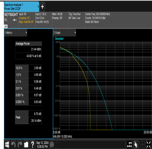
Band26(824-849)-15MHz-16QAM-26915-1RB#0-PASS
