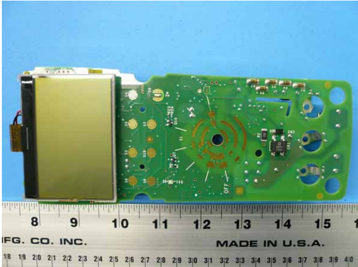
Figure 1: DMM3000 FC Main PCB – Top Side
