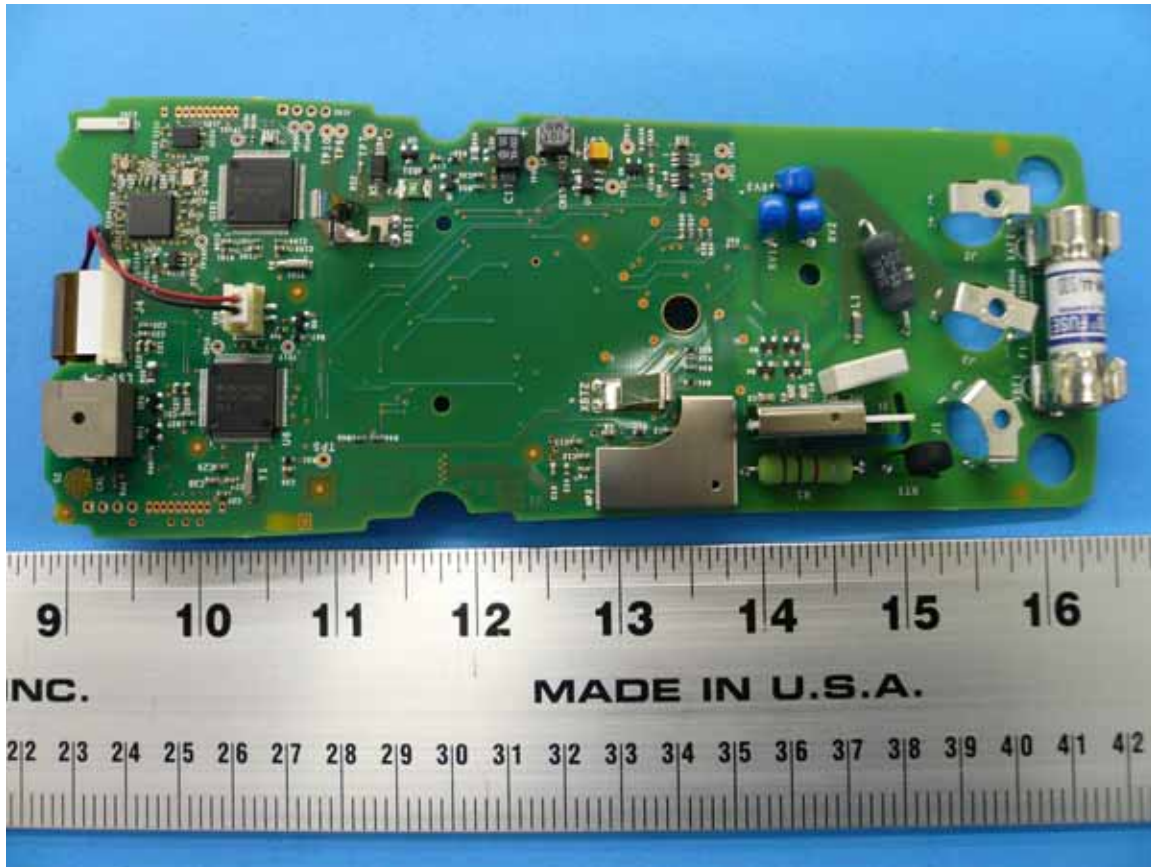
Figure 2: DMM3000 FC Main PCB – Bottom Side
