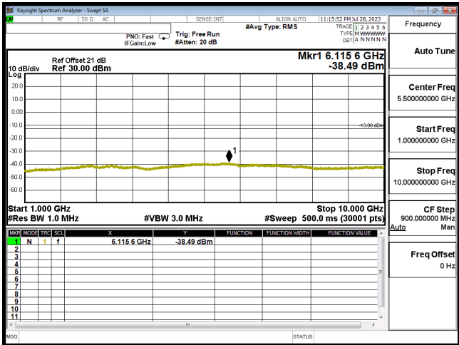
CSE B26 10M CH26740 QPSK(1,25) 1G-10G
