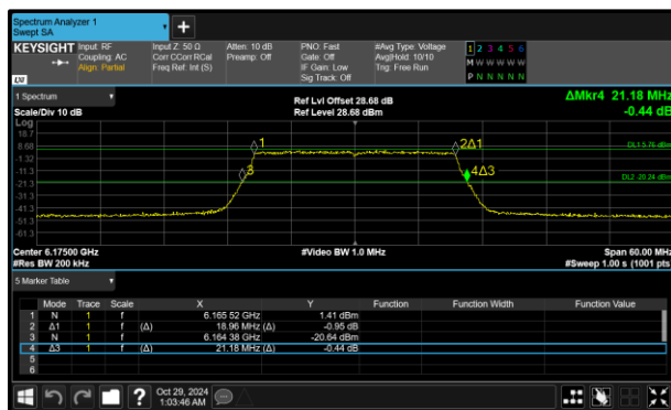
Figure 147 - 802.11ax HE20 SU SP Minimum 26 dB EBW
