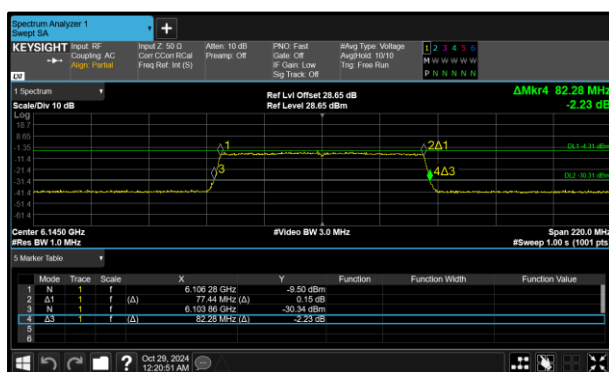
Figure 145 - 802.11ax HE80 SU LPI Minimum 26 dB EBW
