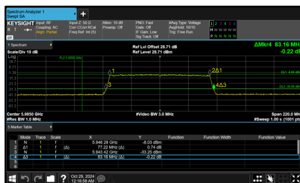
Figure 146 - 802.11ax HE80 SU LPI Maximum 26 dB EBW
