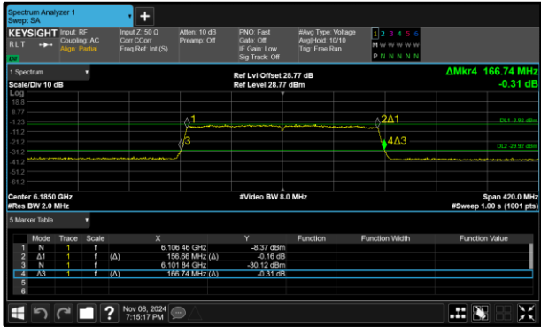
Figure 99 - 802.11ax HE160 SU VLP Minimum 99% OBW
