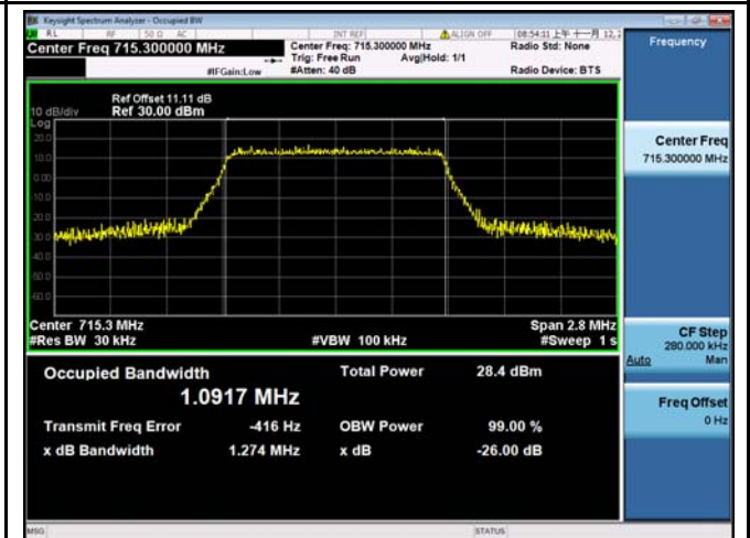
LTE band 12 - High CH 16QAM-1.4
