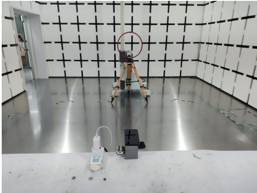
Radiation (9KHz-30MHz)
