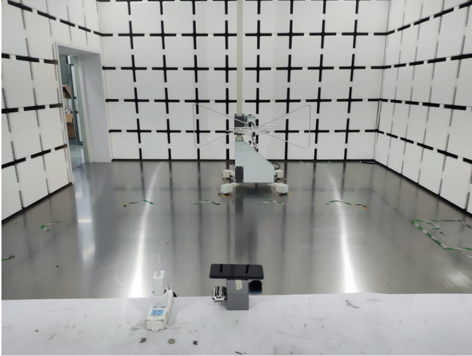
Radiation (30MHz-1000MHz)
