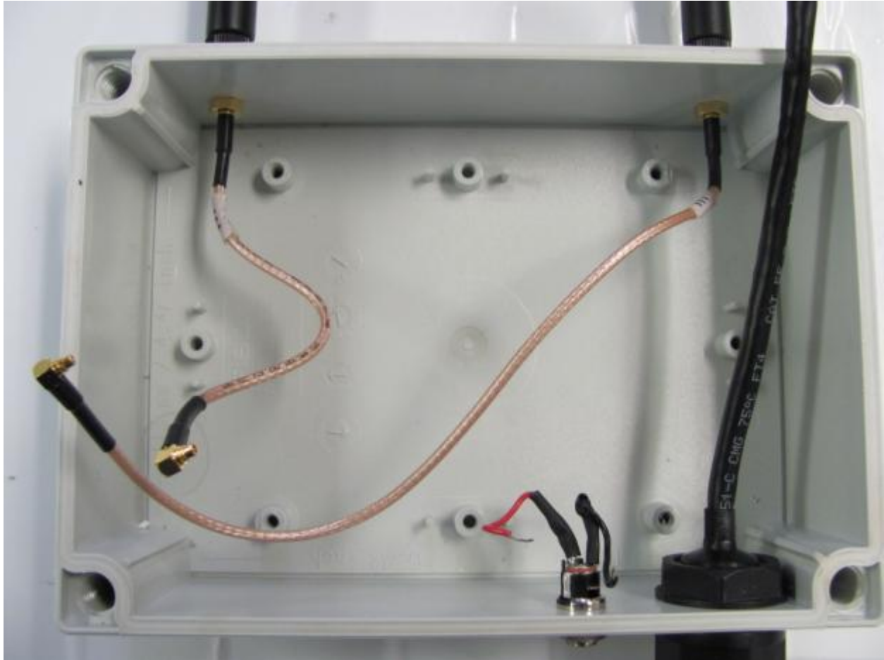
Figure 11. Empty Enclosure
