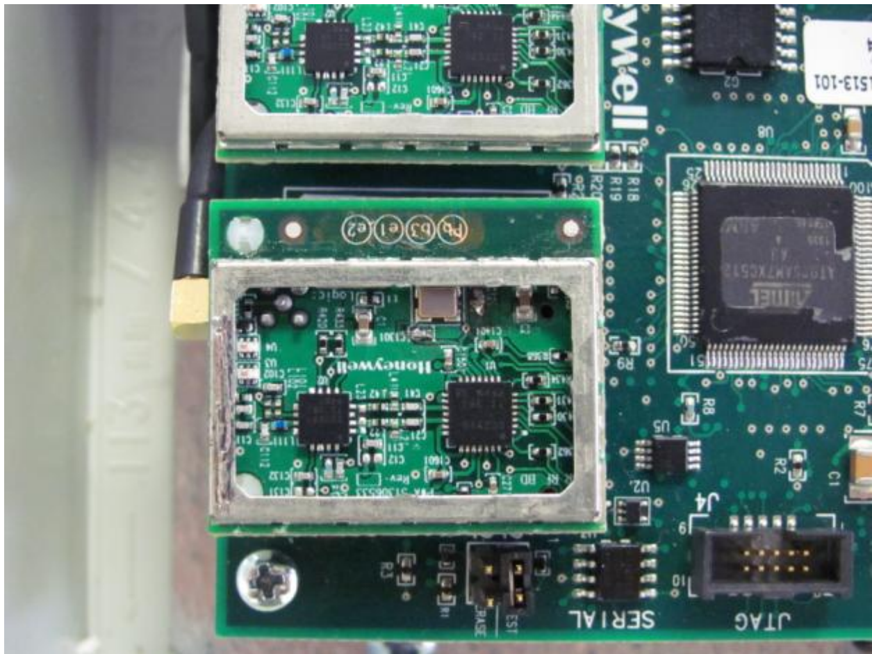
Figure 3. Radio 2 with Shielding Removed
