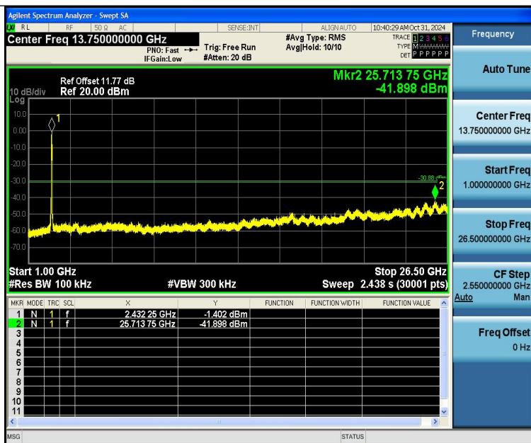
11N40SISO-Ant1-2437-1000~26500-PASS
