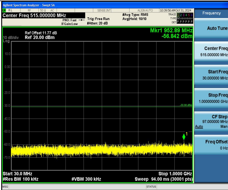
11N40SISO-Ant1-2437-30~1000-PASS
