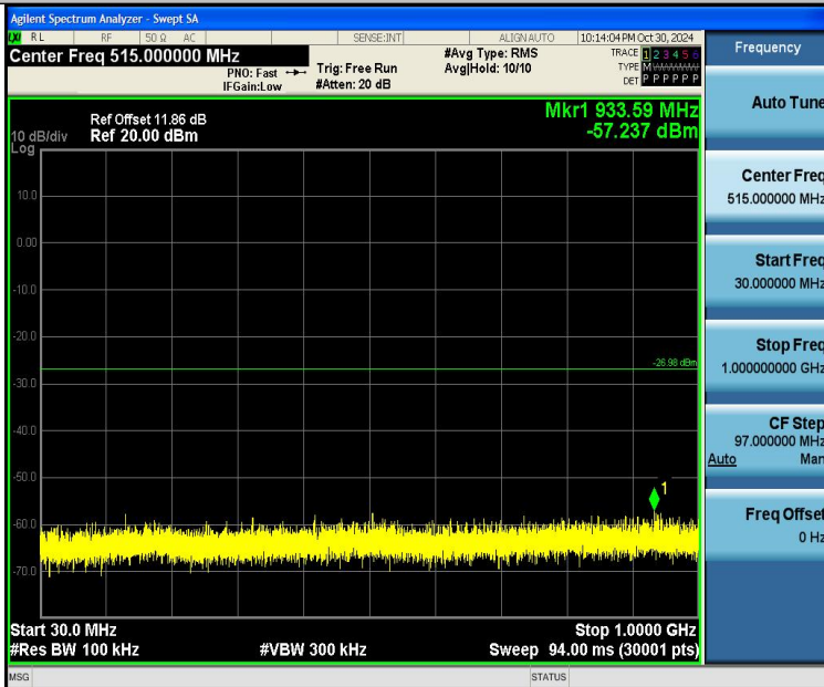
11N20SISO-Ant1-2462-30~1000-PASS
