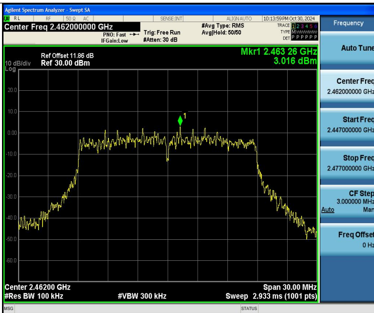
11N20SISO-Ant1-2462-0~Reference-PASS
