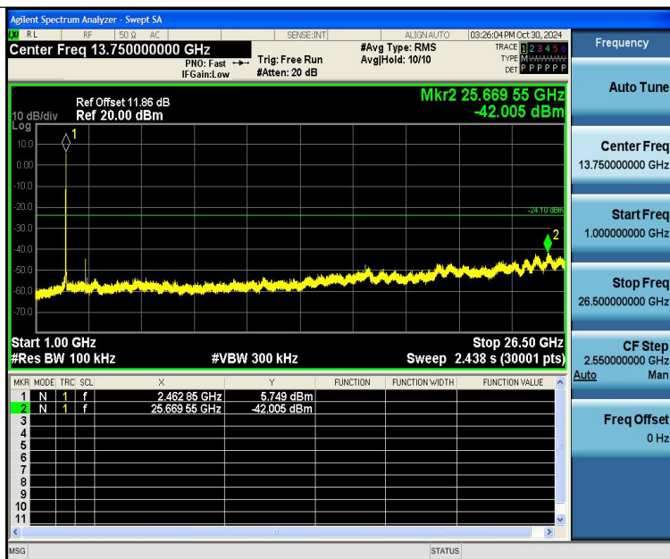
11B-Ant1-2462-1000~26500-PASS
