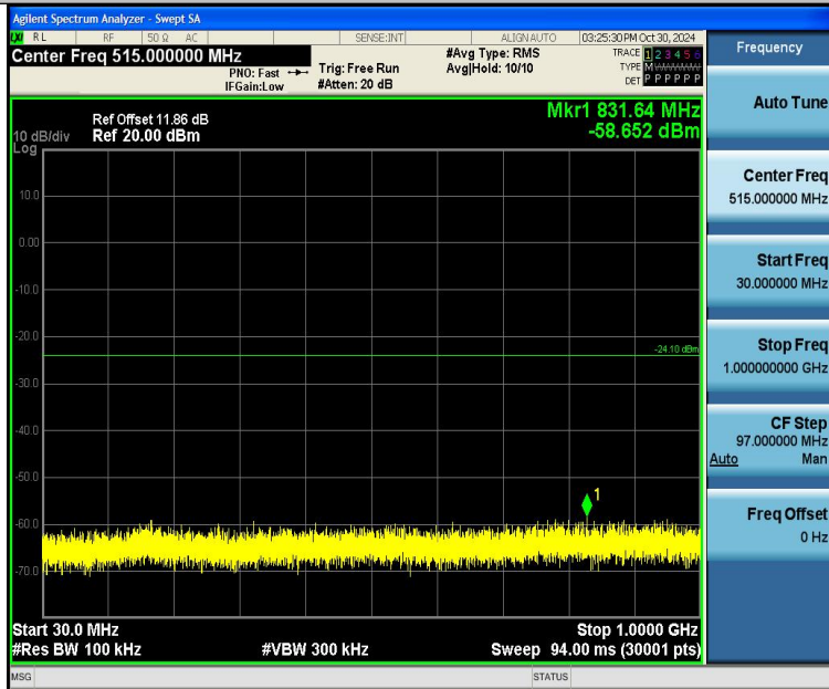
11B-Ant1-2462-30~1000-PASS
