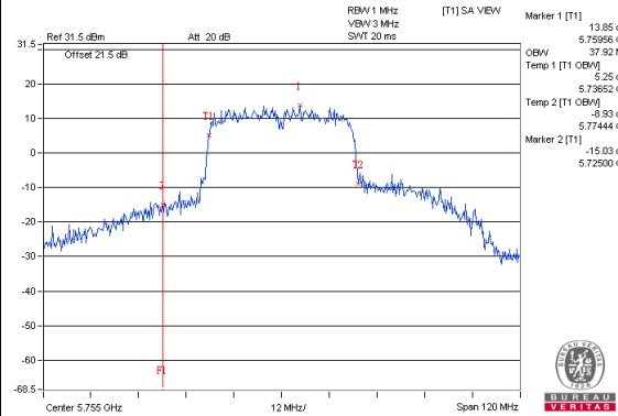
802.11ac(VHT40)_Chain1 / CH151
