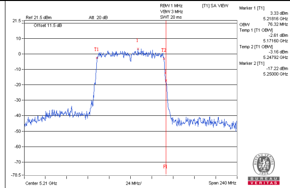
802.11ac(VHT80) / CH42
