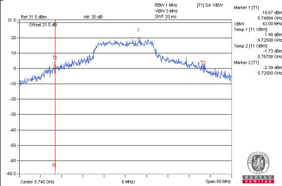
802.11ac(VHT20)_Chain0 / CH149
