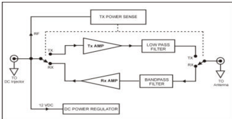
Model 2440 Functional Block Diagram
