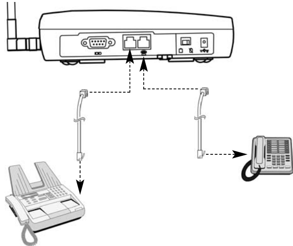
Figure 12 - Dual Jack mode connections.
