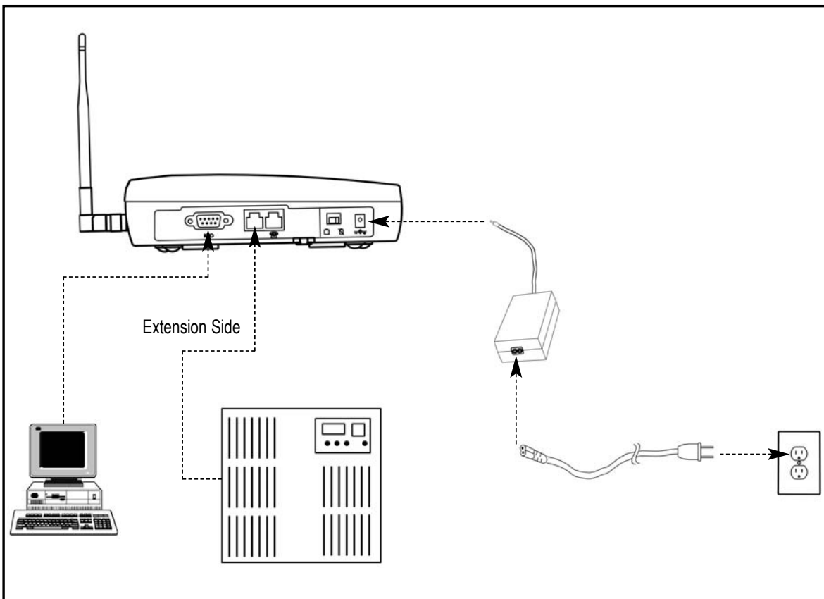
SX5e Fixed Wireless PBX Terminal (attached to Extension side of PBX)
