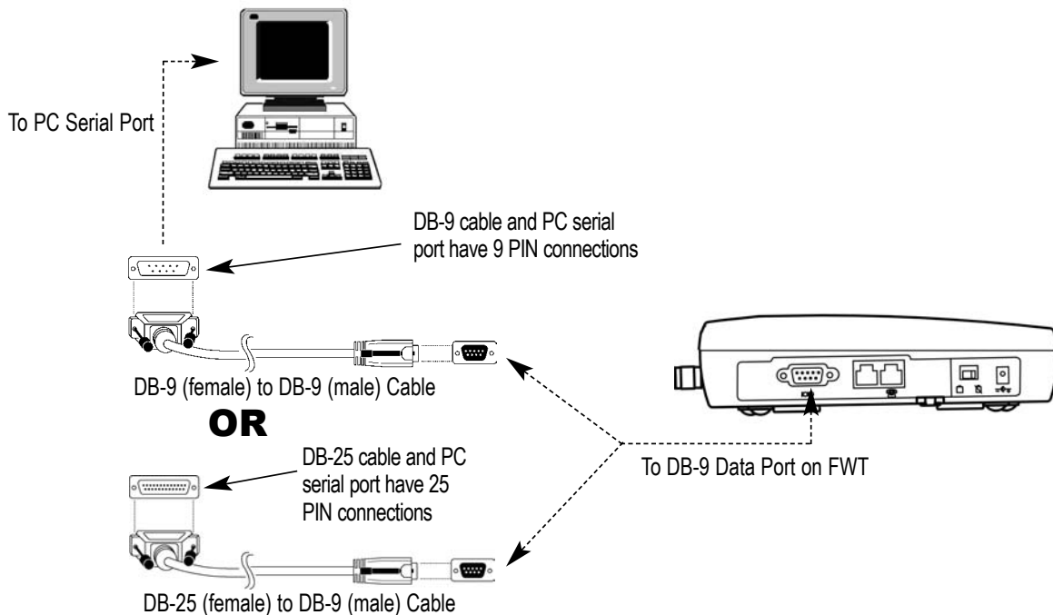
Figure 11 - PC data connection.
