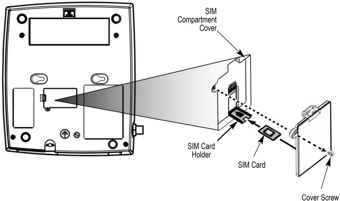
Figure 1 - SIM compartment.
