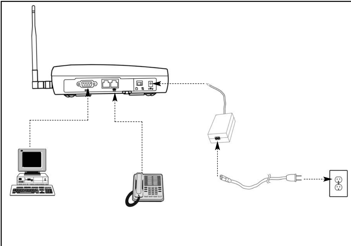
SX5e Fixed Wireless Terminal
