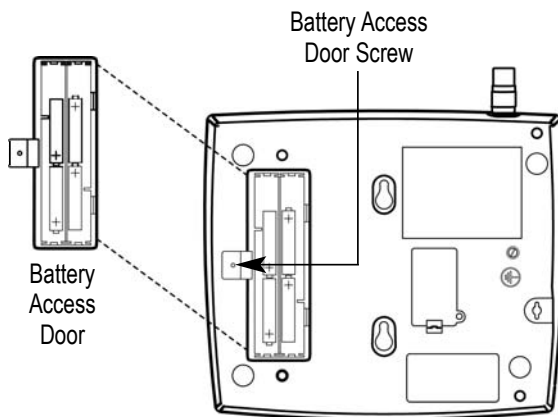
Figure 3 – SX5e battery installation.
