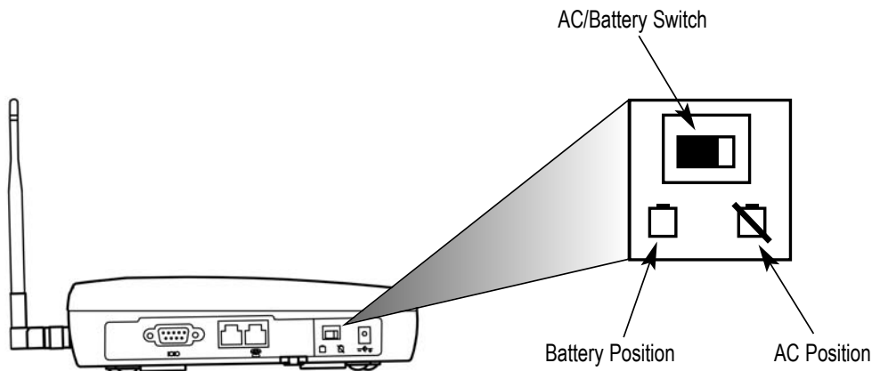
Figure 4 – SX5e AC/Battery switch.
