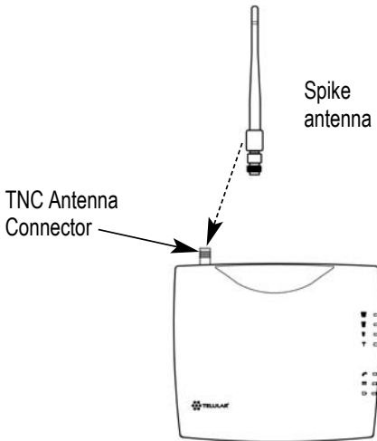
Figure 5 – SX5e antenna connection.
