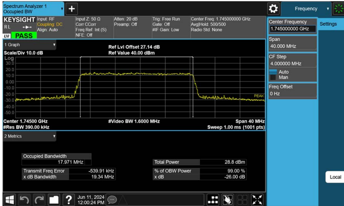
Sub6 n66_20 M_OBW_Mid_64QAM_FullRB
