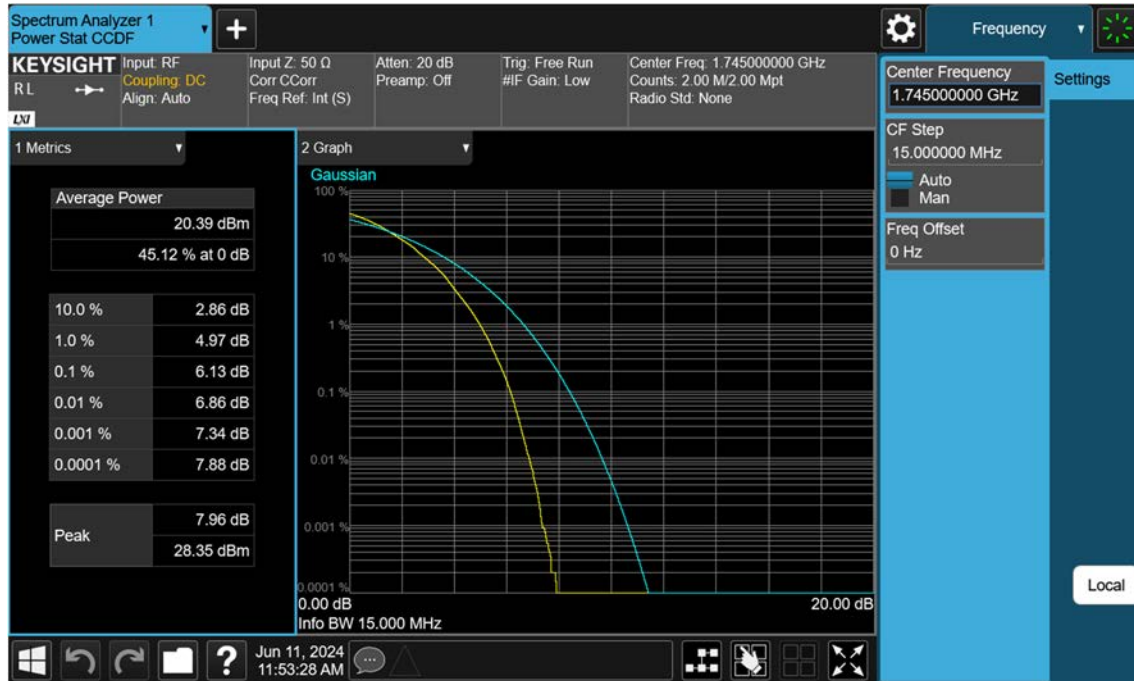
Sub6 n66_15 M_PAR_Mid_64QAM_FullRB
