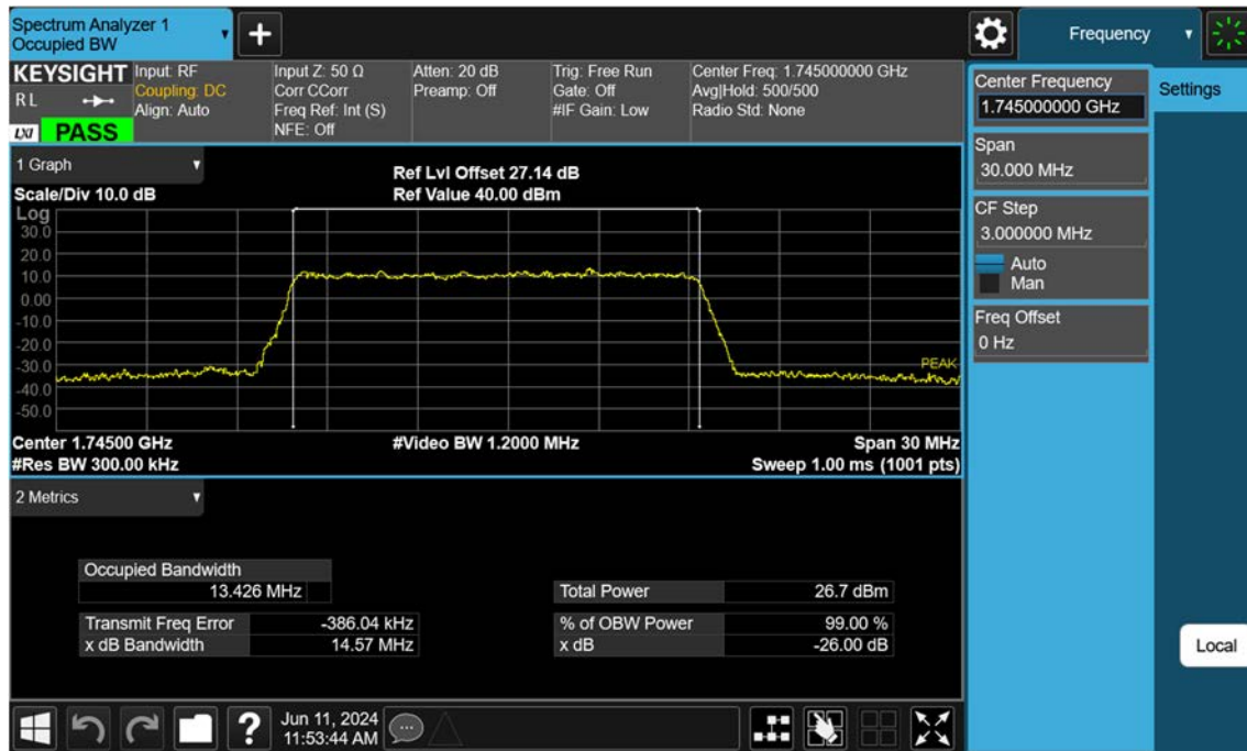
Sub6 n66_15 M_OBW_Mid_256QAM_FullRB
