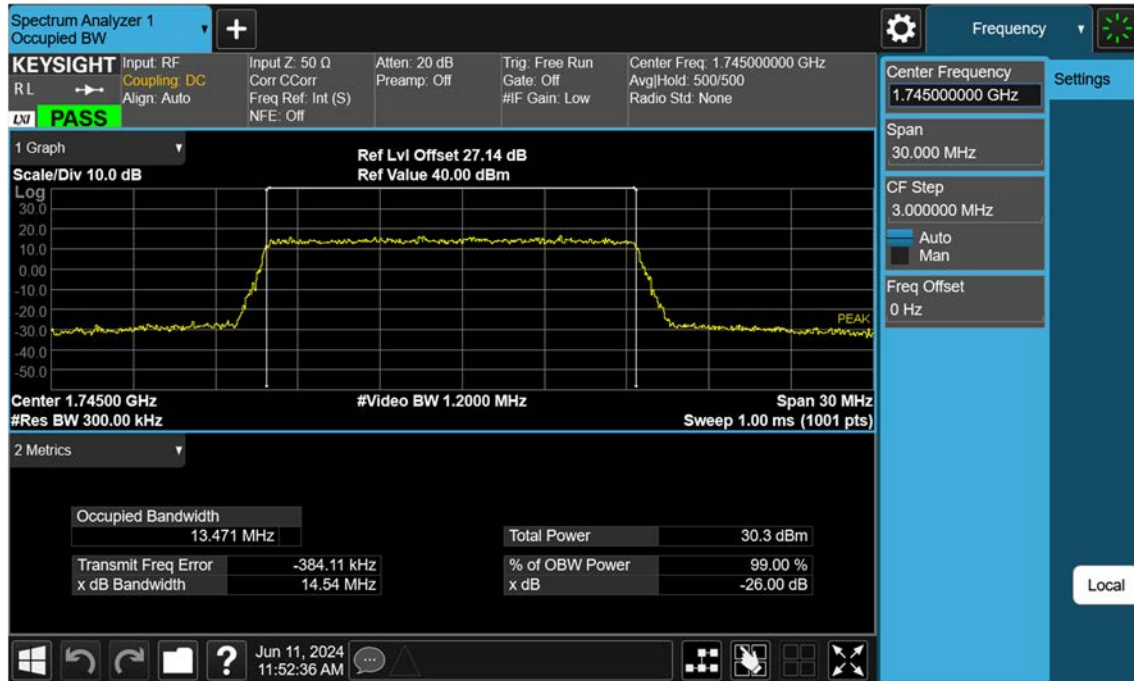
Sub6 n66_15 M_OBW_Mid_QPSK_FullRB
