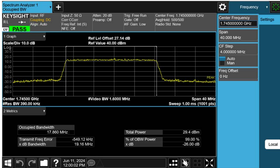
Sub6 n66_20 M_OBW_Mid_16QAM_FullRB
