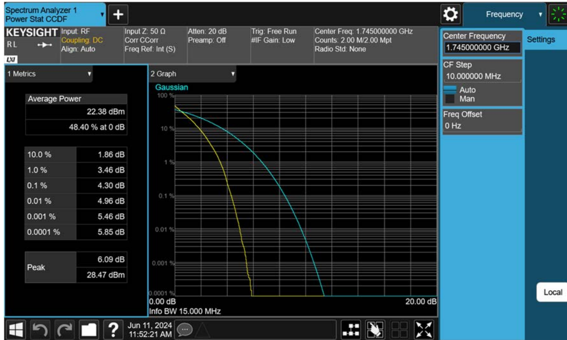
Sub6 n66_15 M_PAR_Mid_BPSK_FullRB
