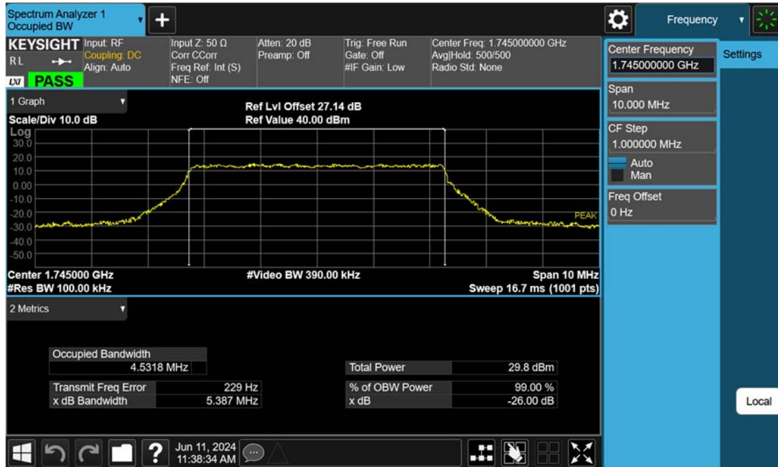
Sub6 n66_5 M_OBW_Mid_16QAM_FullRB
