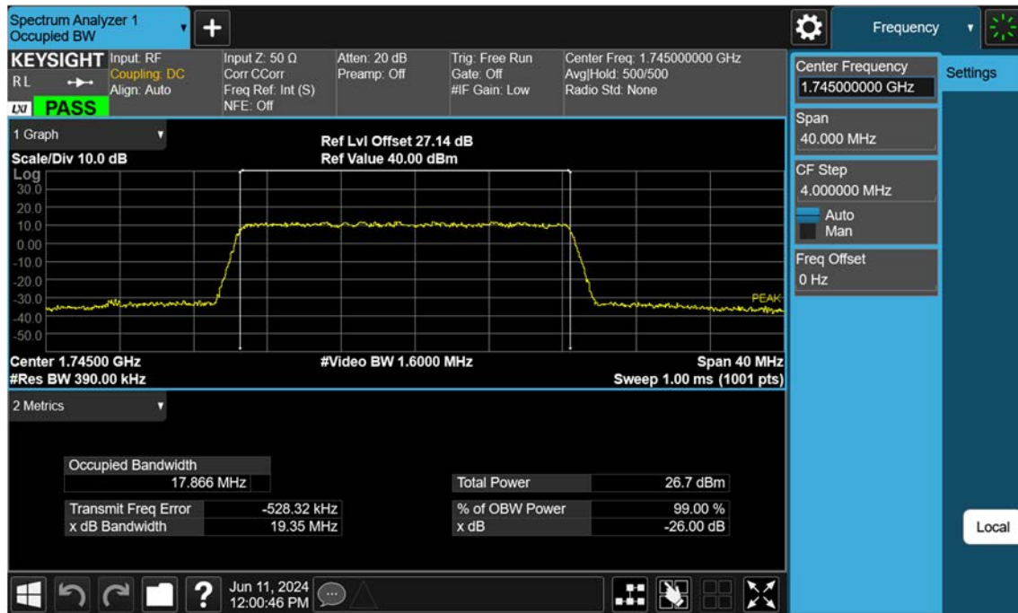
Sub6 n66_20 M_OBW_Mid_256QAM_FullRB
