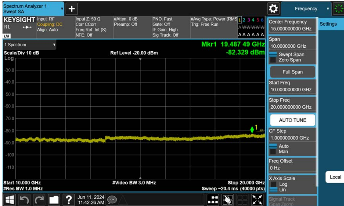
Sub6 n66_5 M_Conducted Spurious(Above10 G)_High_BPSK_1RB
