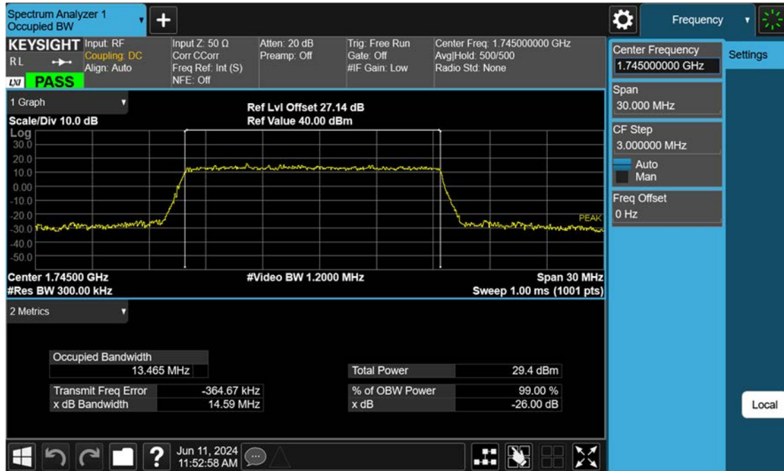
Sub6 n66_15 M_OBW_Mid_16QAM_FullRB
