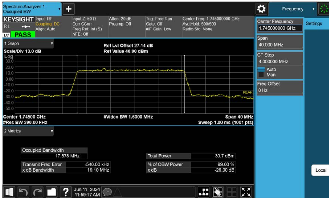
Sub6 n66_20 M_OBW_Mid_BPSK_FullRB
