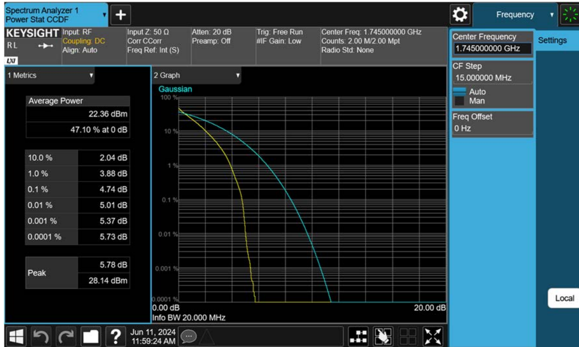
Sub6 n66_20 M_PAR_Mid_BPSK_FullRB
