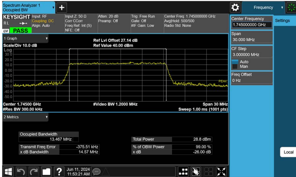
Sub6 n66_15 M_OBW_Mid_64QAM_FullRB
