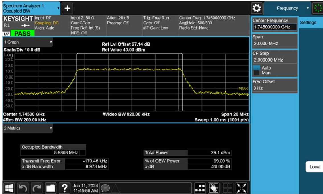
Sub6 n66_10 M_OBW_Mid_16QAM_FullRB
