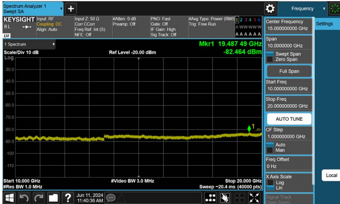
Sub6 n66_5 M_Conducted Spurious(Above10 G)_Mid_BPSK_1RB
