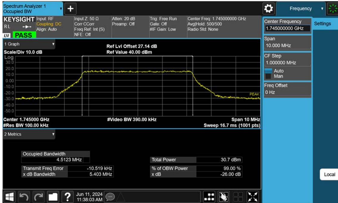
Sub6 n66_5 M_OBW_Mid_QPSK_FullRB
