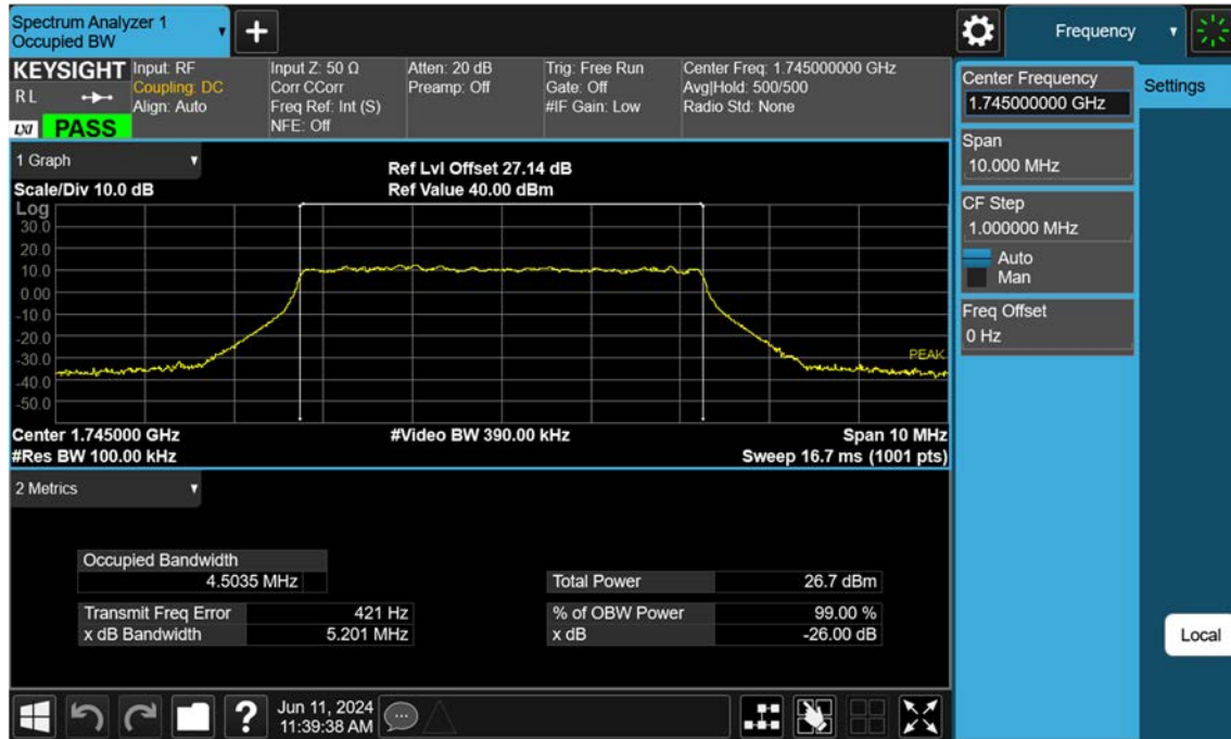
Sub6 n66_5 M_OBW_Mid_256QAM_FullRB
