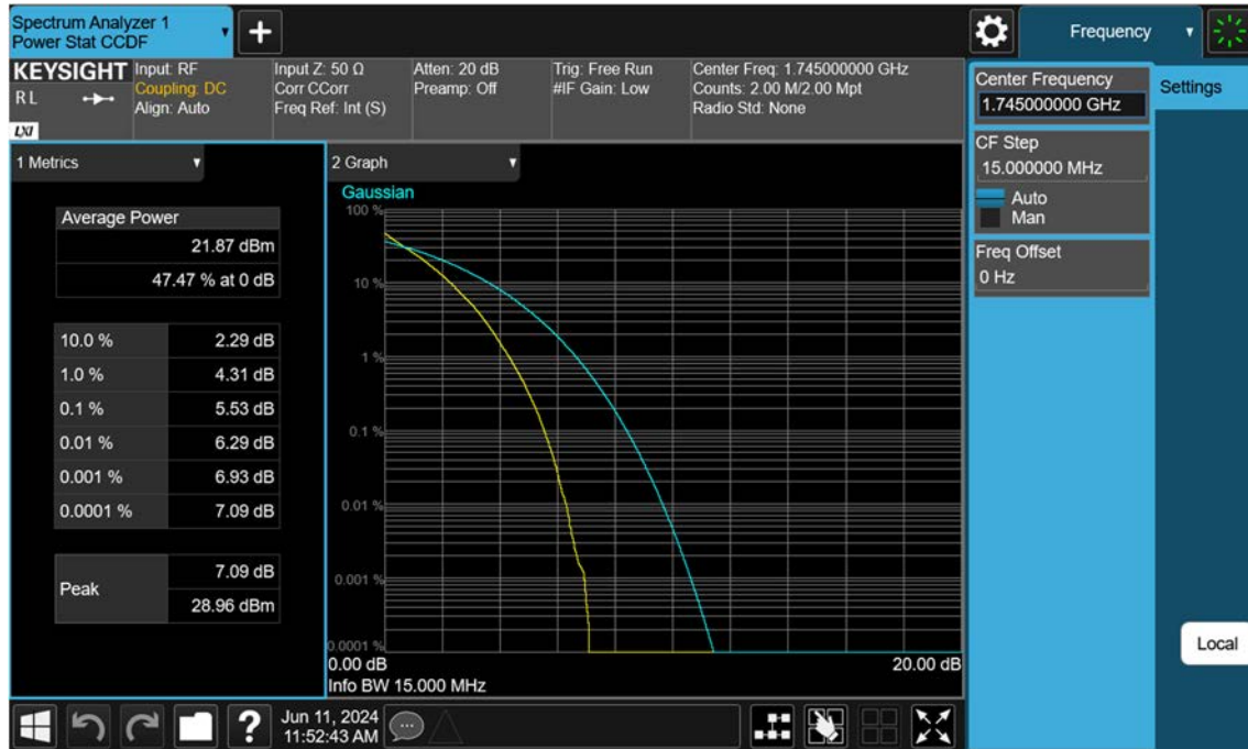
Sub6 n66_15 M_PAR_Mid_QPSK_FullRB
