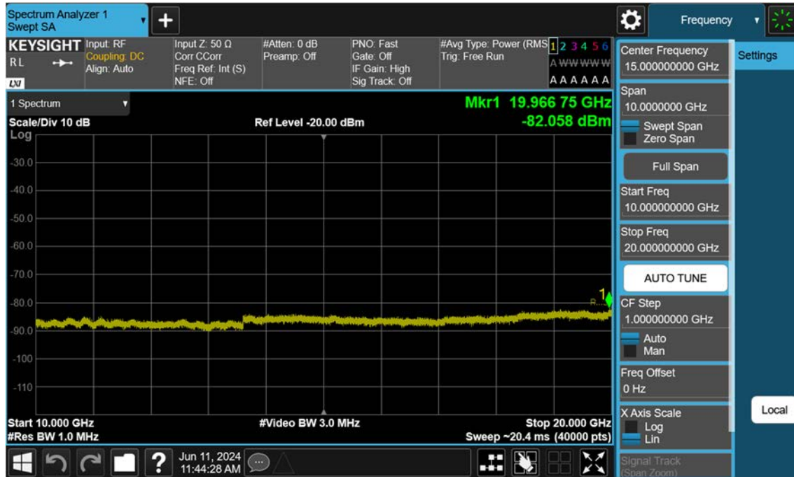
Sub6 n66_10 M_Conducted Spurious(Above10 G)_Low_BPSK_1RB
