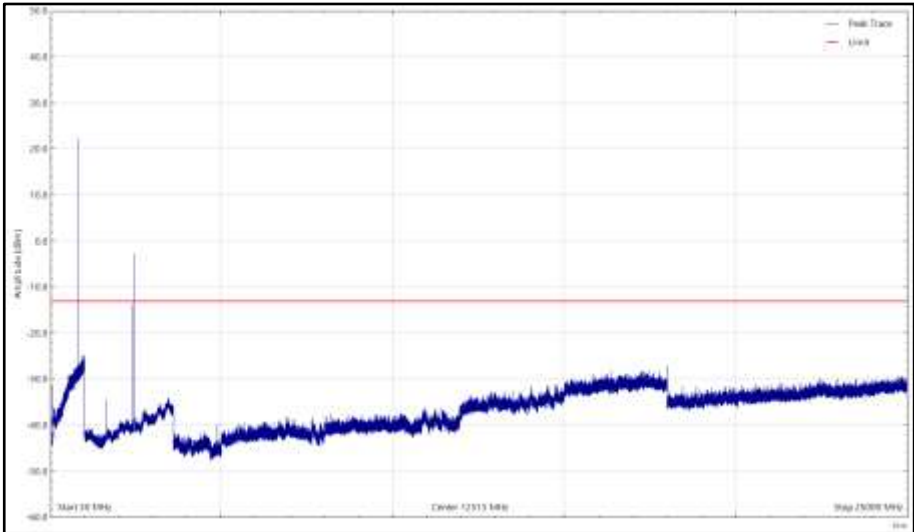
Figure 8 - 30 MHz to 25 GHz, Vertical – X Orientation (ISED)
