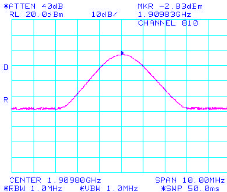
Figure 31: High Channel PCS Peak power
