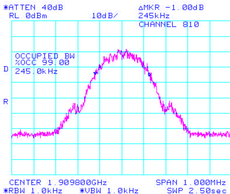
Figure 3: High Channel PCS Occupied Bandwidth (99%)
