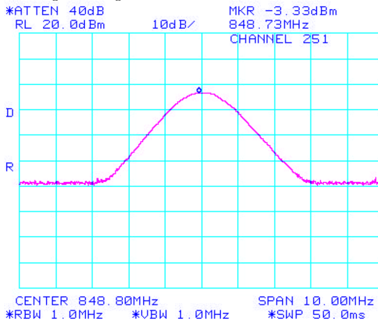
Figure 34: High Channel GSM850 Peak Power
