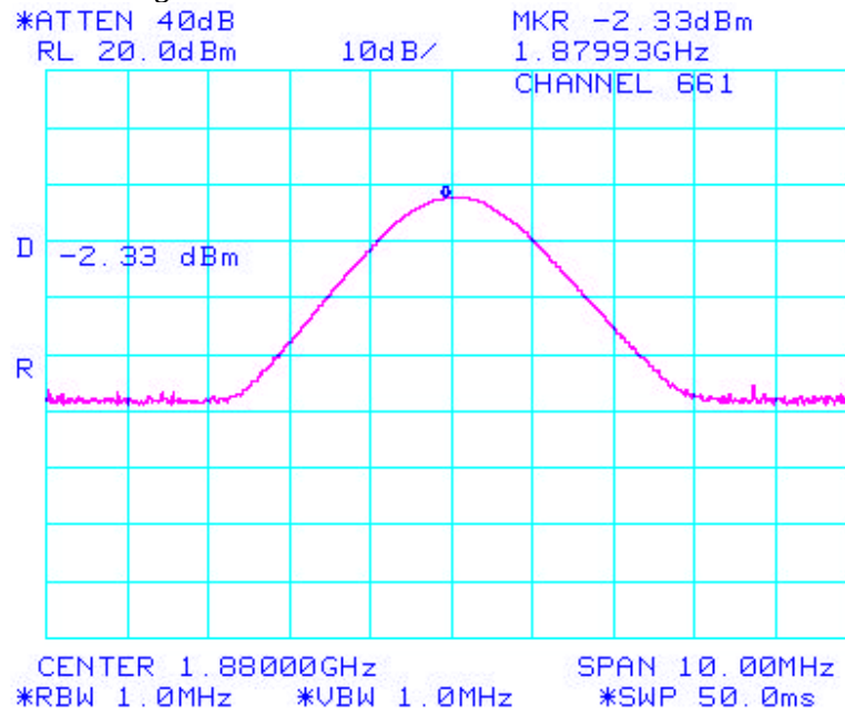
Figure 30: Middle Channel PCS Peak Power
