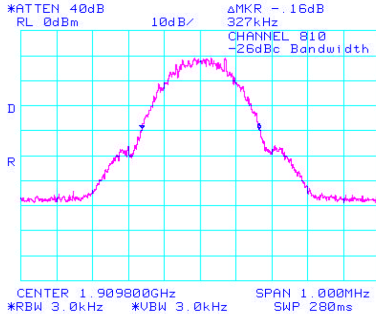
Figure 9: High Channel PCS -26 dBc Bandwidth (99%)
