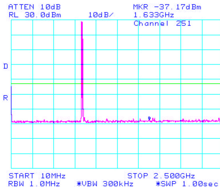
Figure 23: GSM850 High Channel, Spurious Emissions
