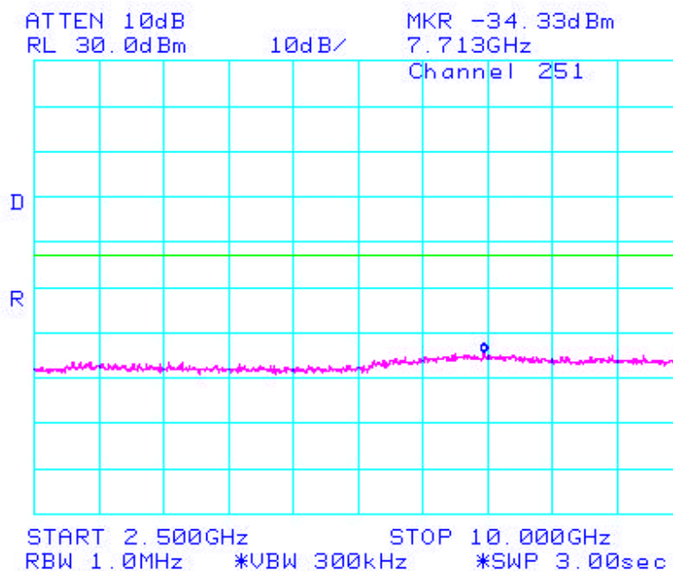
Figure 24: GSM850 High Channel, Spurious Emissions
