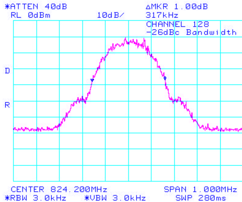
Figure 10: Low Channel GSM850 -26 dBc Bandwidth
