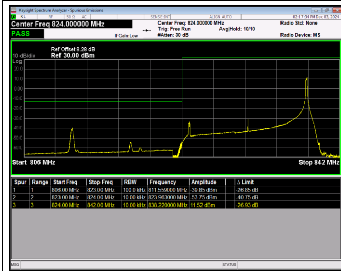
Band26-15MHz-QPSK-26965-1RB#0
