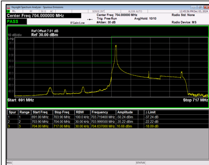
Band17-10MHz-16QAM-23780-50RB#0
