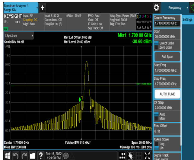
Band66-10MHz-QPSK-132022-1-0-Low--30.60-PASS
