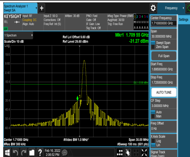
Band66-15MHz-QPSK-132047-1-0-Low--31.27-PASS
