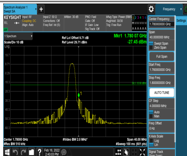
Band66-20MHz-QPSK-132572-6-0-High--27.45-PASS
