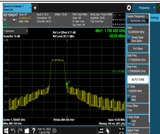
Band66-5MHz-QPSK-132647-6-0-High--30.05-PASS
