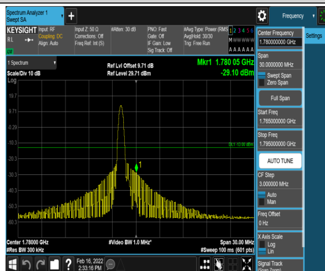
Band66-15MHz-QPSK-132597-1-0-High--29.10-PASS
