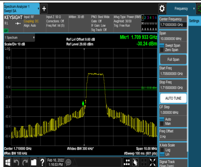
Band66-5MHz-QPSK-131997-6-0-Low--30.24-PASS
