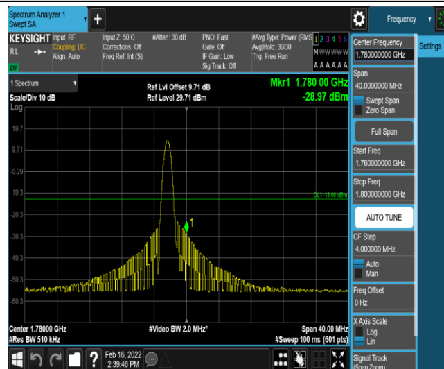
Band66-20MHz-QPSK-132572-1-0-High--28.97-PASS
