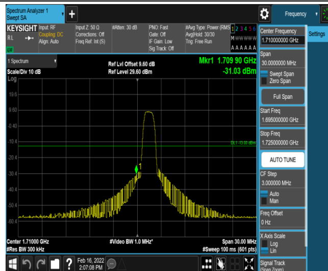
Band66-15MHz-QPSK-132047-6-0-Low--31.03-PASS
