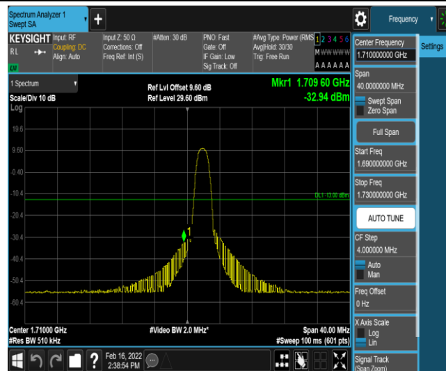
Band66-20MHz-QPSK-132072-6-0-Low--32.94-PASS
