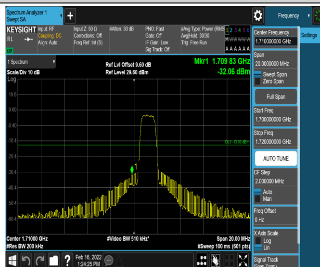
Band66-10MHz-QPSK-132022-6-0-Low--32.06-PASS
