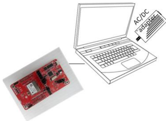
Figure 3.6-1: Setup diagram
