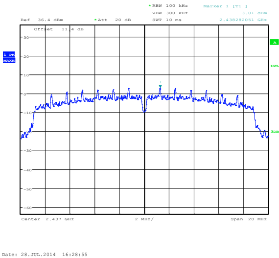
Figure 8.6-3: PSD sample plot on 802.11n
