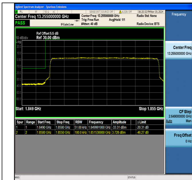
Band2 5MHz 16QAM 18625 25RB#0
