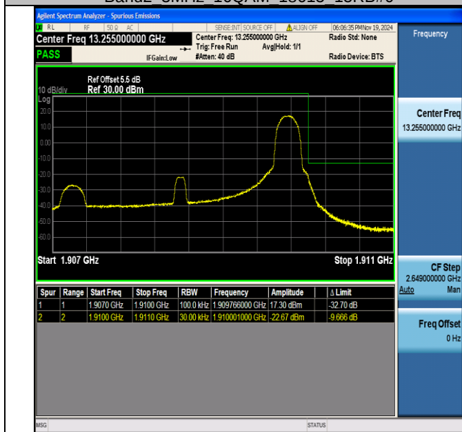
Band2 3MHz 16QAM 19185 1RB#14
