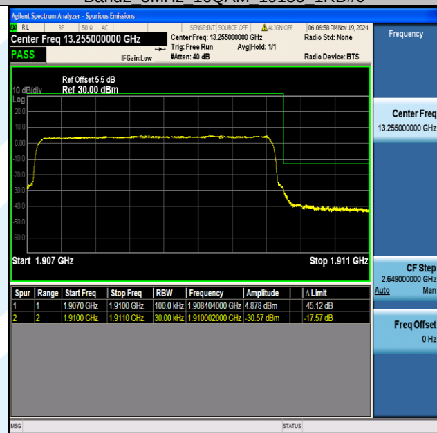
Band2 3MHz 16QAM 19185 15RB#0
