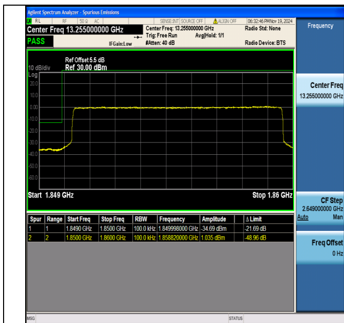
Band2 10MHz 16QAM 18650 50RB#0
