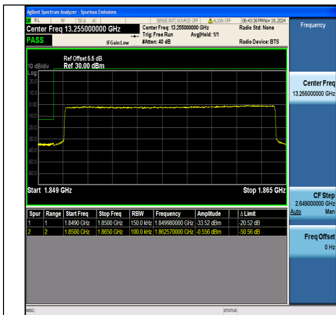
Band2 15MHz 16QAM 18675 75RB#0
