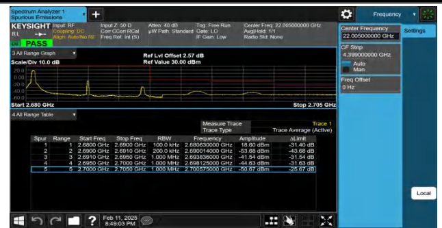
Band41-10MHz-QPSK-41540-1RB#0-PASS
