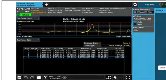
Band41-5MHz-QPSK-39675-1RB#0-PASS
