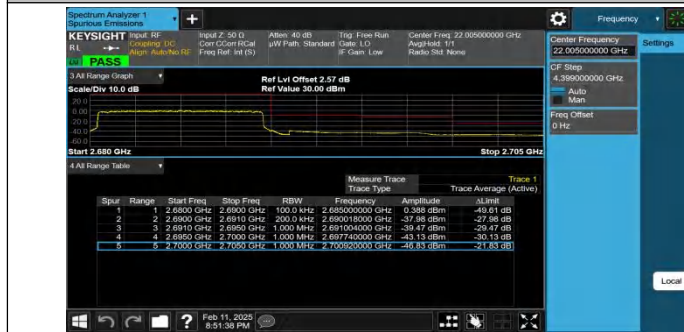
Band41-10MHz-QPSK-41540-50RB#0-PASS
