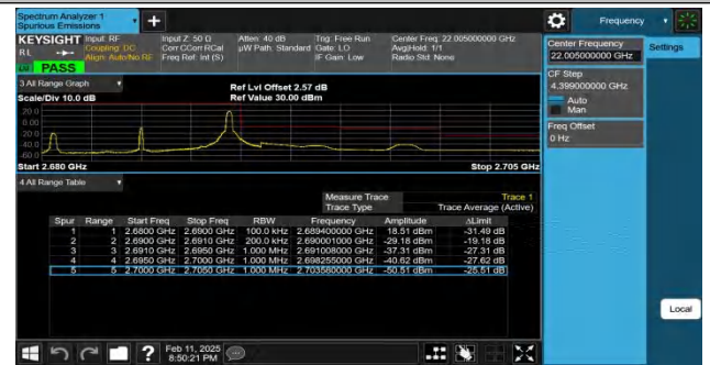
Band41-10MHz-QPSK-41540-1RB#49-PASS
