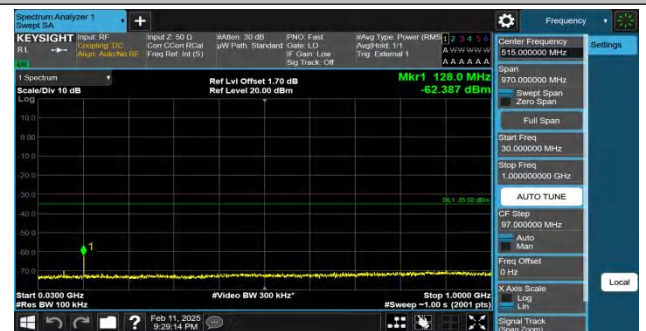
Band41-15MHz-QPSK-41515-1RB#74-30~1000-PASS
