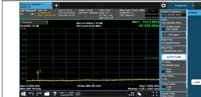
Band41-15MHz-QPSK-41515-1RB#0-30~1000-PASS
