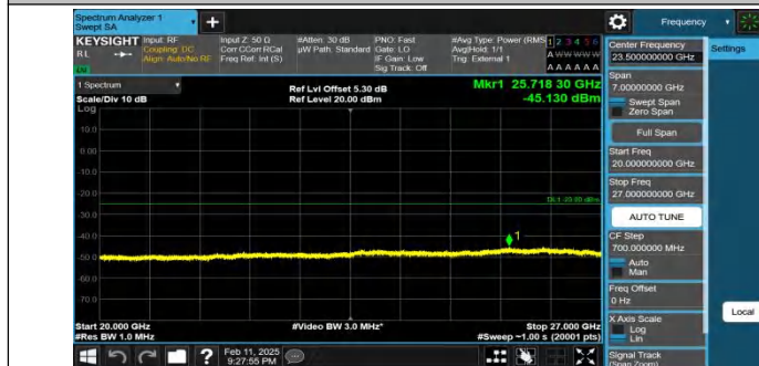
Band41-15MHz-QPSK-41515-1RB#0-20000~27000-PASS
