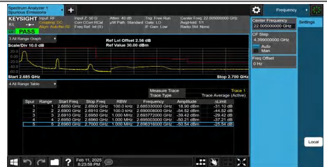
Band41-5MHz-QPSK-41565-1RB#0-PASS
