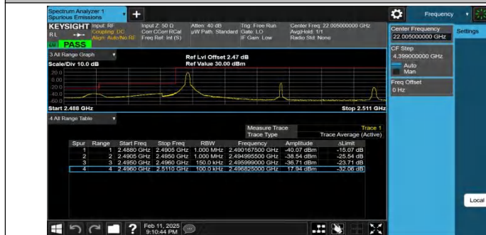
Band41-15MHz-QPSK-39725-1RB#0-PASS
