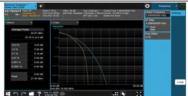
Band41-15MHz-16QAM-40620-75RB#0-PASS
