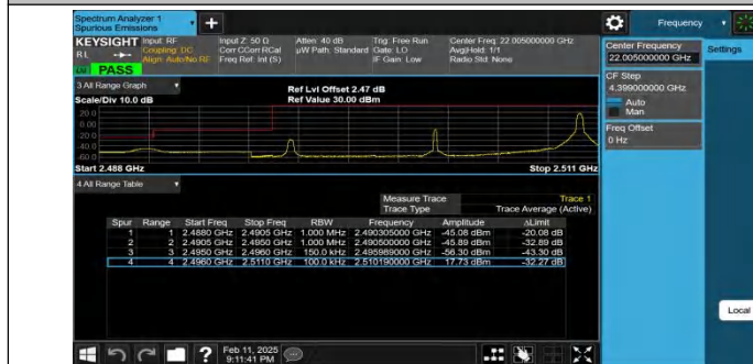
Band41-15MHz-QPSK-39725-1RB#74-PASS
