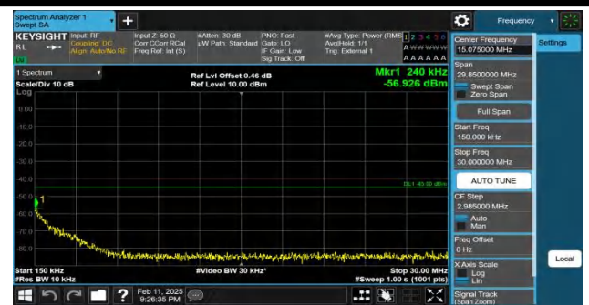
Band41-15MHz-QPSK-41515-1RB#0-0.15~30-PASS
