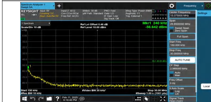
Band41-15MHz-QPSK-39725-1RB#74-0.15~30-PASS
