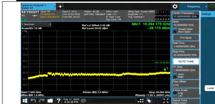
Band41-5MHz-QPSK-39675-1RB#24-1000~20000-PASS
