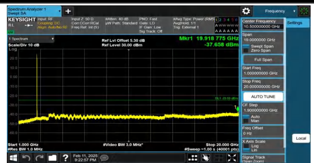
Band41-15MHz-QPSK-40620-1RB#0-1000~20000-PASS
