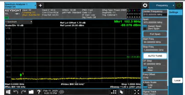
Band41-15MHz-QPSK-39725-1RB#74-30~1000-PASS
