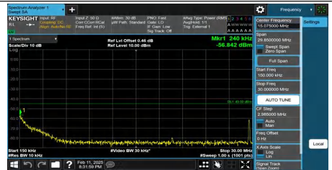
Band41-5MHz-QPSK-40620-1RB#0-0.15~30-PASS
