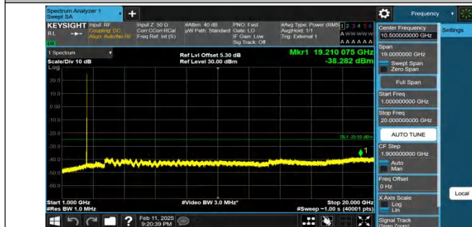
Band41-15MHz-QPSK-39725-1RB#74-1000~20000-PASS
