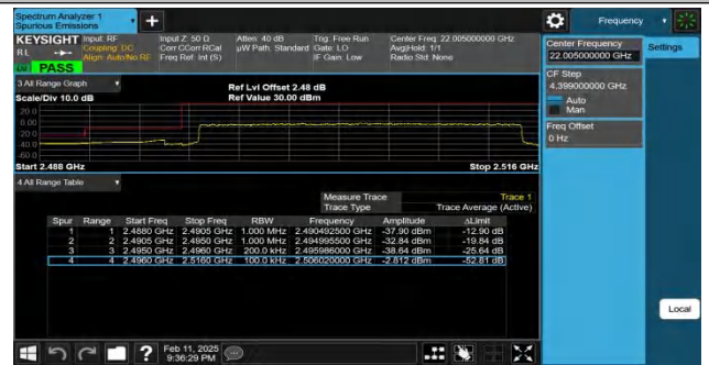
Band41-15MHz-QPSK-41515-1RB#74-PASS
