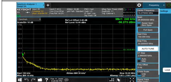
Band41-15MHz-QPSK-41515-1RB#74-0.15~30-PASS
