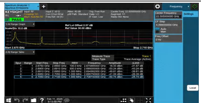
Band41-15MHz-QPSK-41515-1RB#0-PASS
