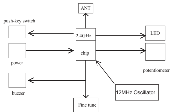
66807TXV1 block diagram
