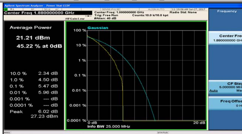
Band2_20MHz_16QAM_18900_100RB#0
