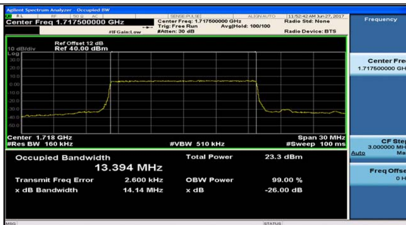
Band4_15MHz_16QAM_20025_75RB#0
