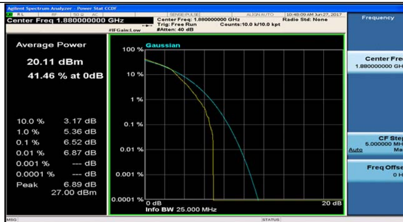
Band2_5MHz_QPSK_18900_25RB#0
