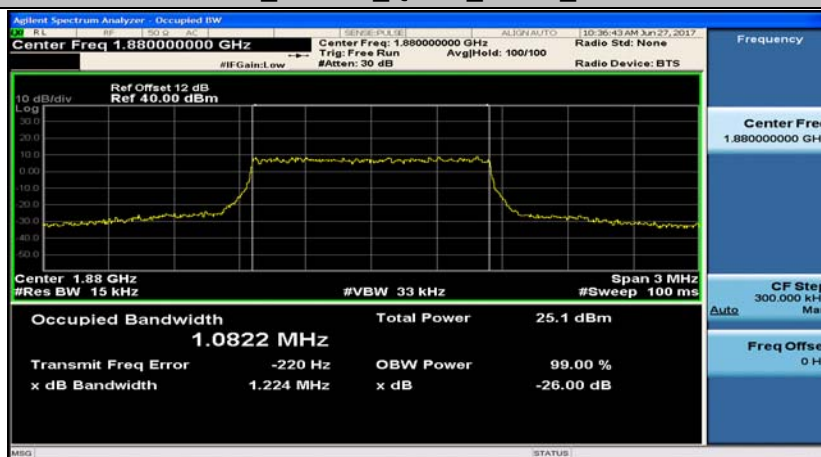
Band2_1.4MHz_16QAM_18900_6RB#0
