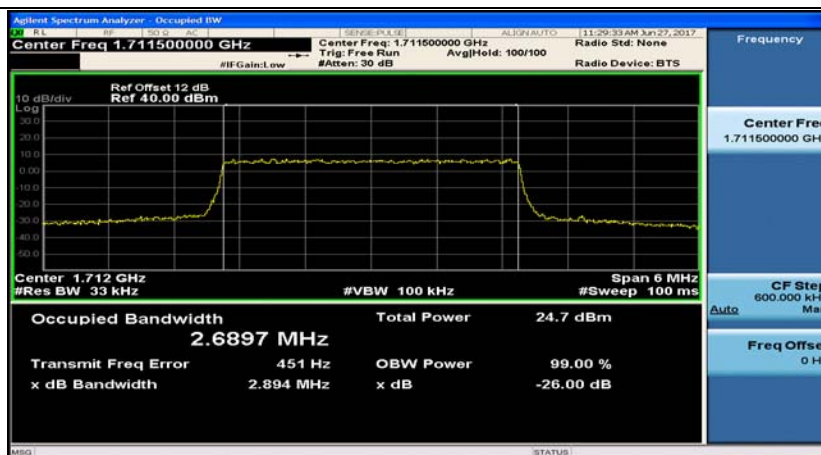
Band4_3MHz_16QAM_19965_15RB#0
