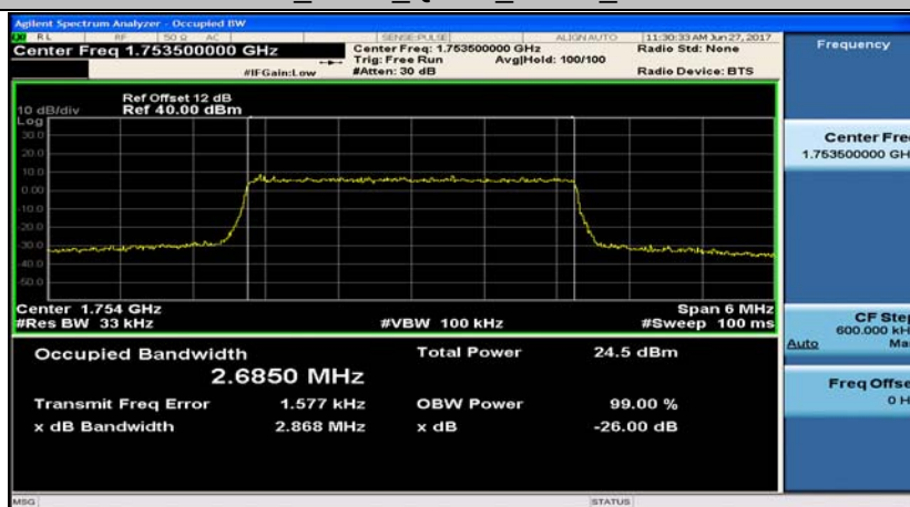
Band4_3MHz_16QAM_20385_15RB#0
