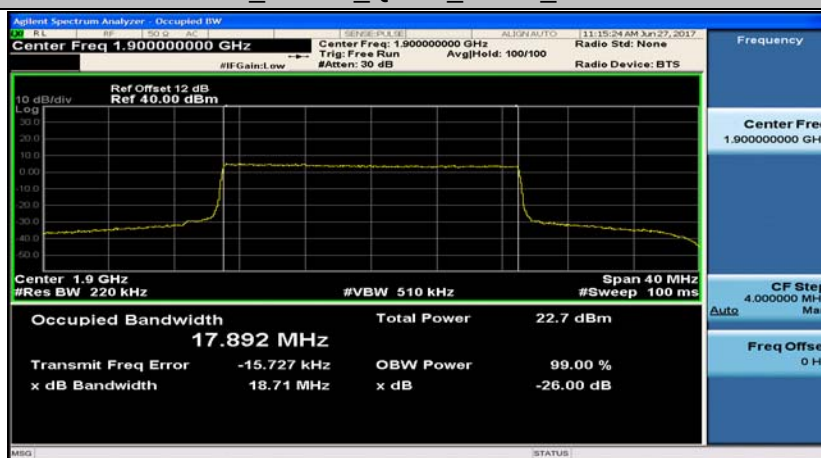
Band2_20MHz_16QAM_19100_100RB#0
