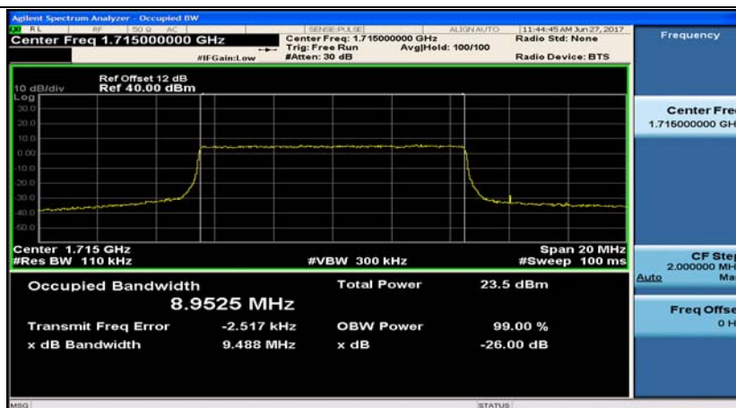
Band4_10MHz_16QAM_20000_50RB#0
