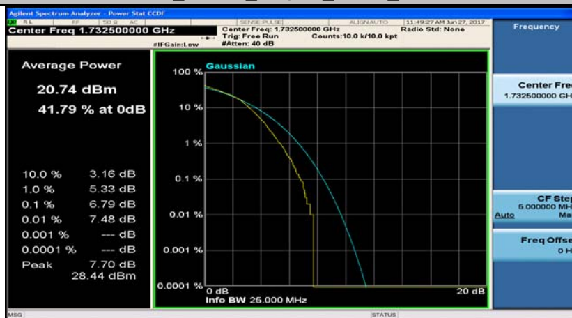
Band4_15MHz_QPSK_20175_75RB#0
