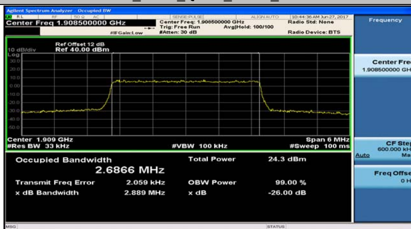
Band2_3MHz_16QAM_19185_15RB#0
