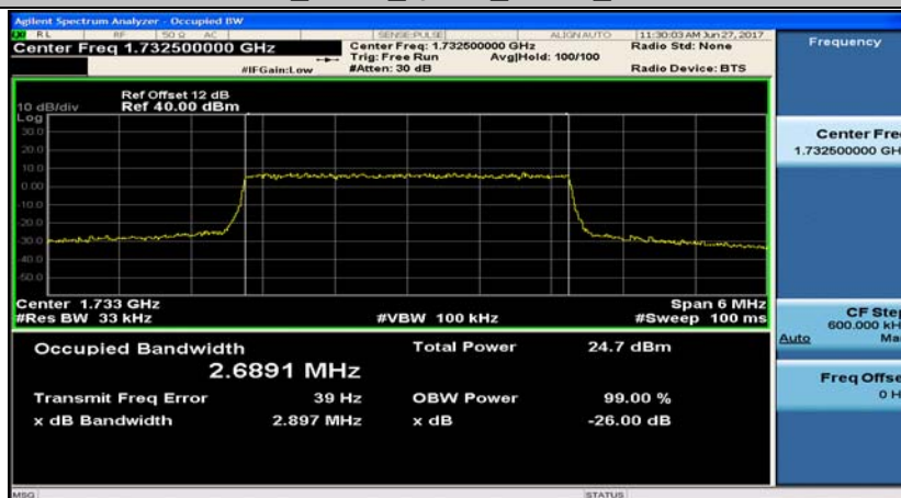
Band4_3MHz_16QAM_20175_15RB#0
