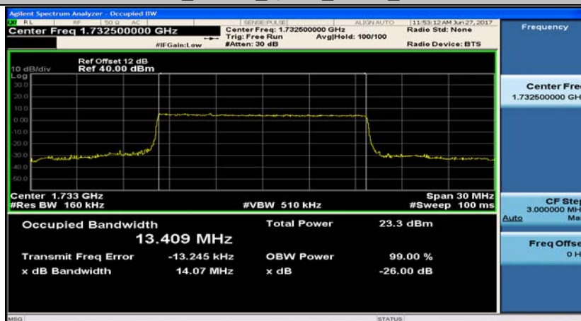
Band4_15MHz_16QAM_20175_75RB#0
