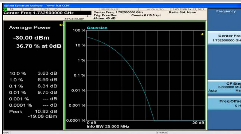
Band4_20MHz_16QAM_20175_100RB#0
