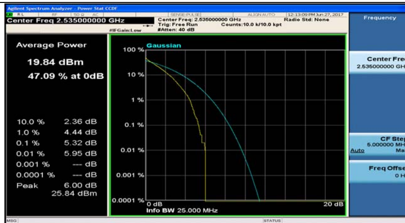
Band7_5MHz_16QAM_21100_25RB#0
