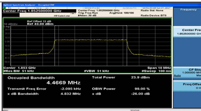
Band2_5MHz_16QAM_18625_25RB#0
