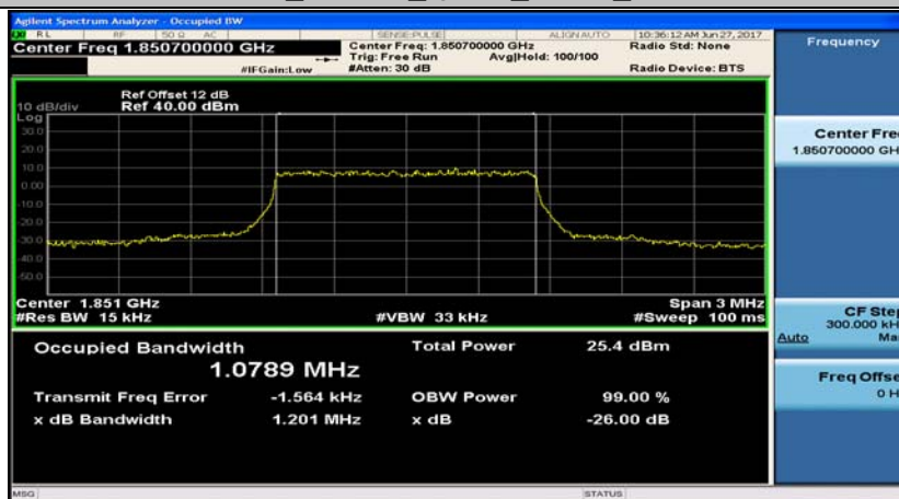
Band2_1.4MHz_16QAM_18607_6RB#0
