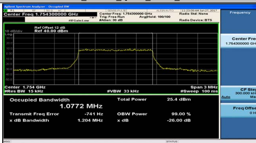
Band4_1.4MHz_16QAM_20393_6RB#0
