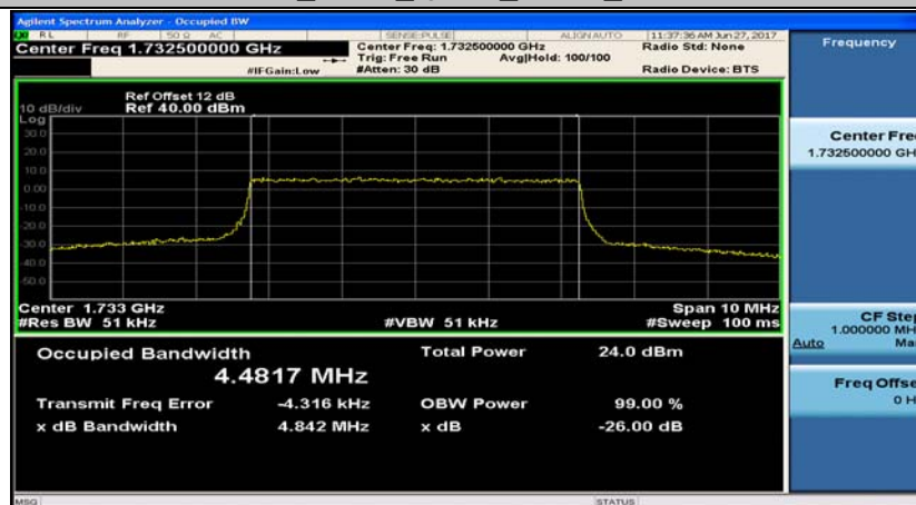
Band4_5MHz_16QAM_20175_25RB#0
