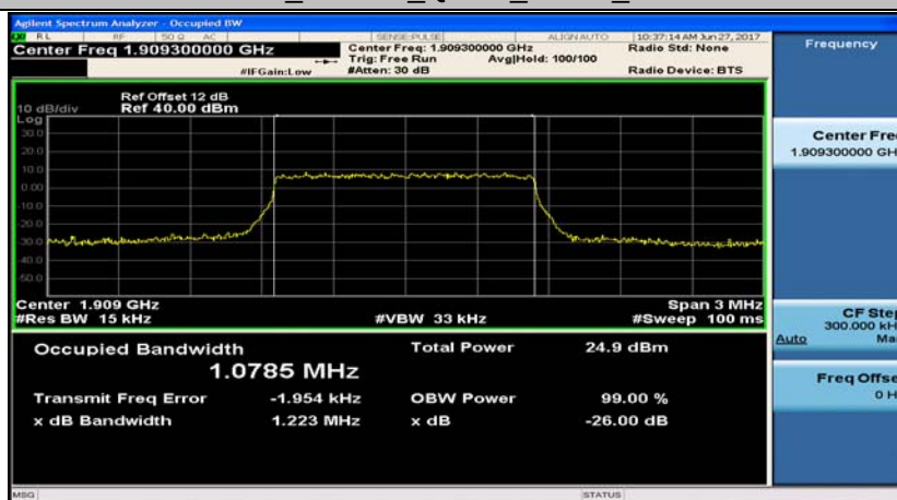
Band2_1.4MHz_16QAM_19193_6RB#0
