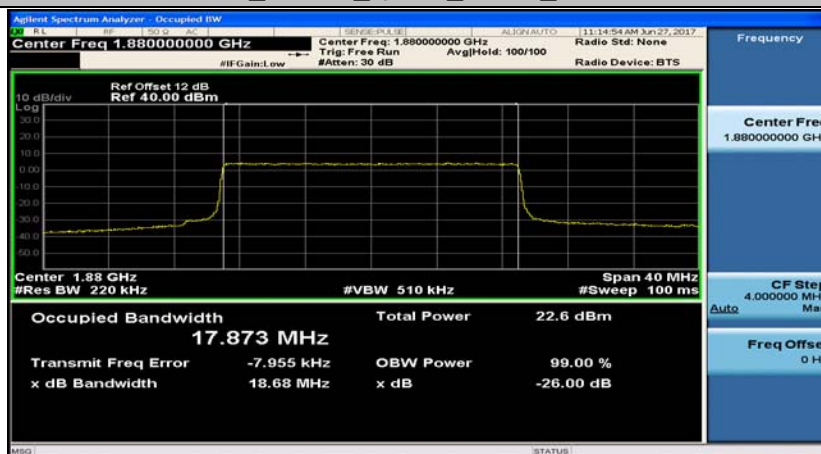
Band2_20MHz_16QAM_18900_100RB#0
