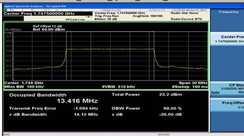
Band4_15MHz_16QAM_20325_75RB#0
