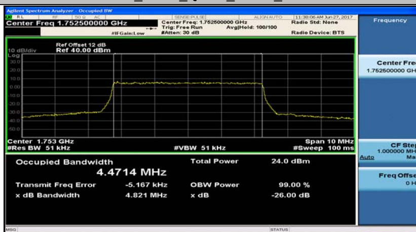
Band4_5MHz_16QAM_20375_25RB#0
