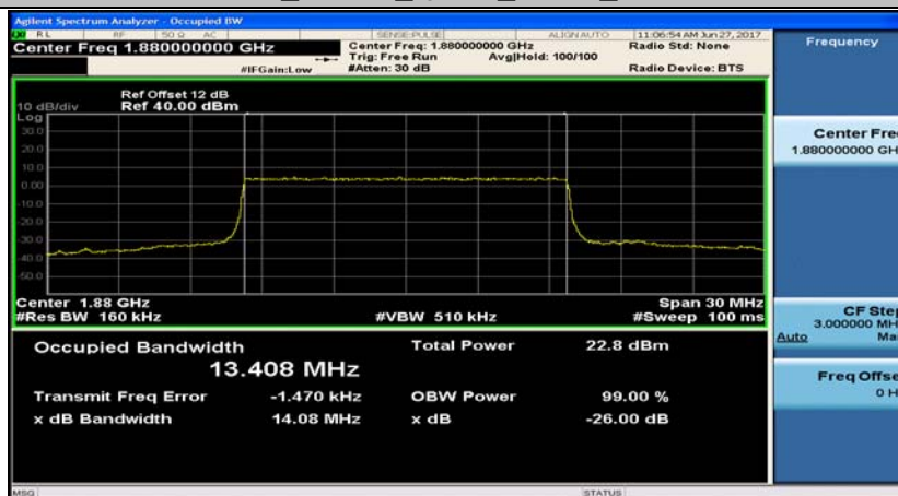
Band2_15MHz_16QAM_18900_75RB#0
