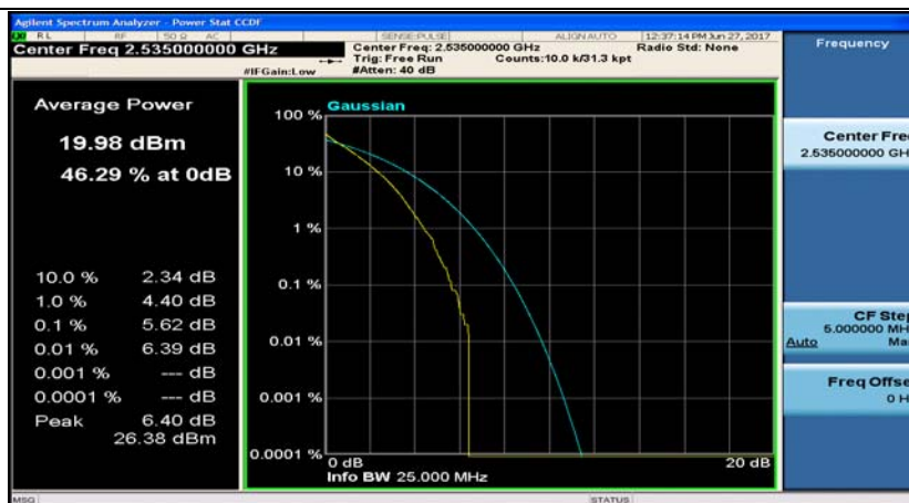
Band7_20MHz_16QAM_21100_100RB#0
