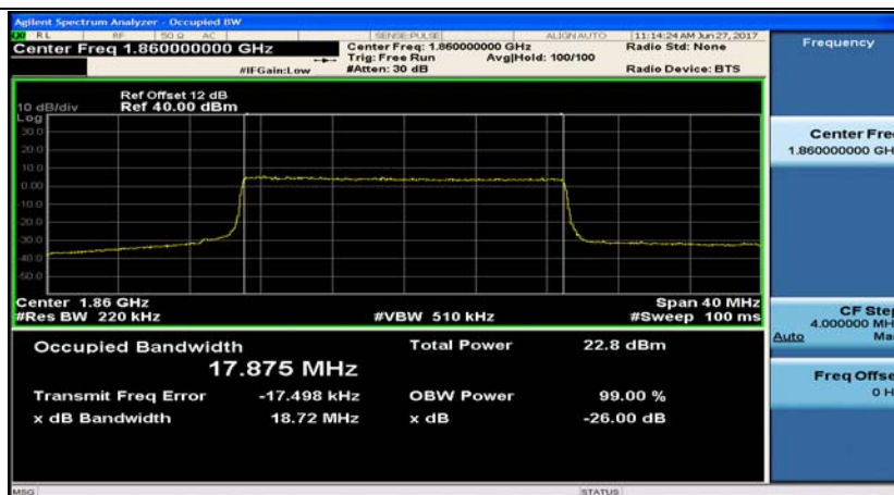
Band2_20MHz_16QAM_18700_100RB#0
