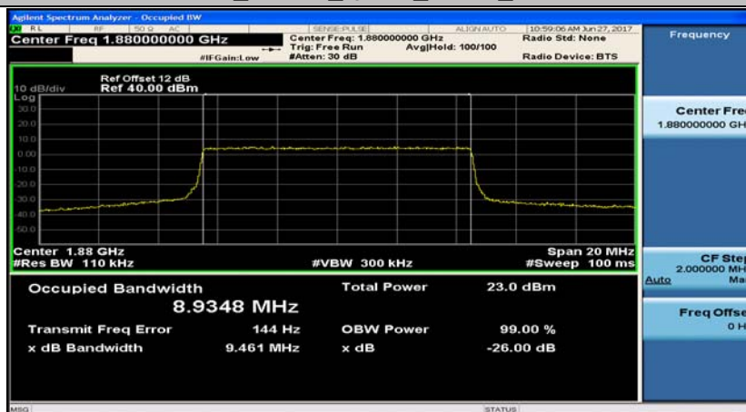
Band2_10MHz_16QAM_18900_50RB#0
