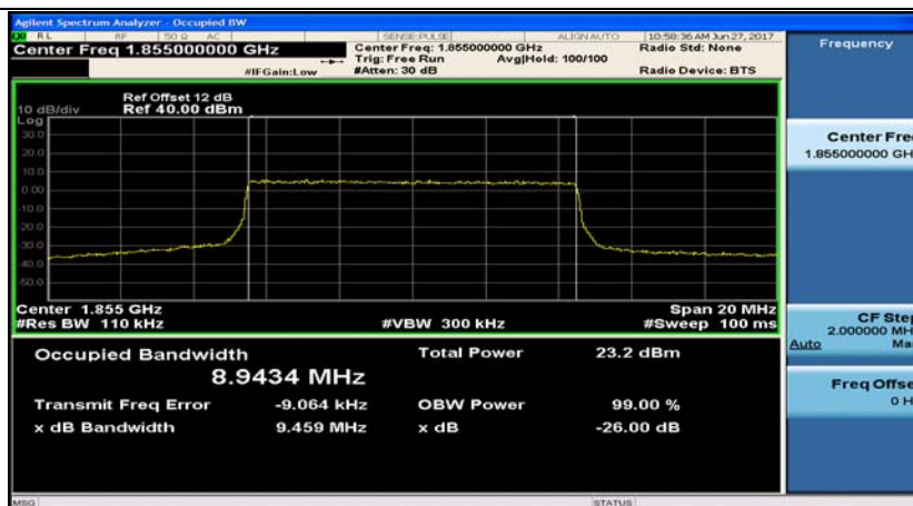
Band2_10MHz_16QAM_18650_50RB#0
