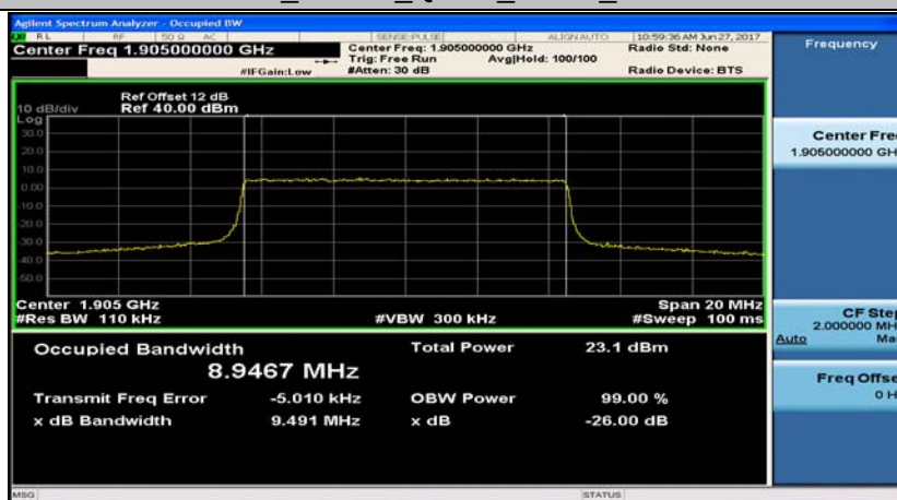
Band2_10MHz_16QAM_19150_50RB#0
