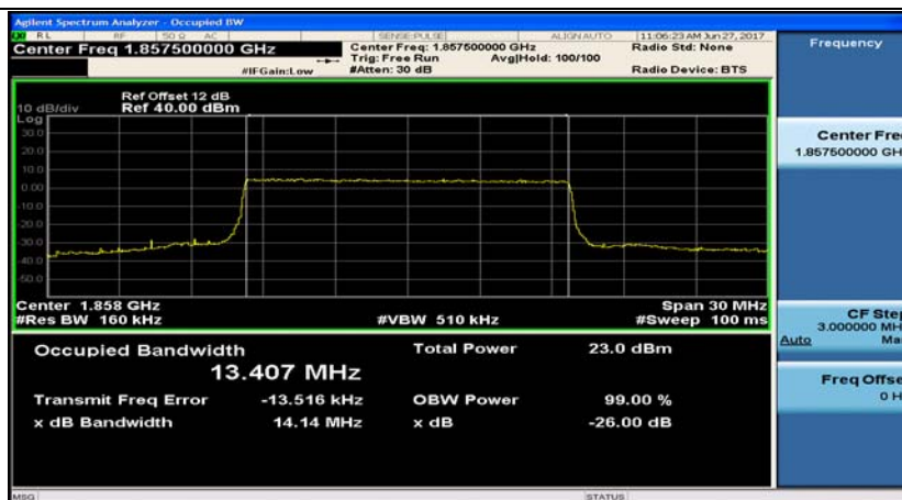
Band2_15MHz_16QAM_18675_75RB#0
