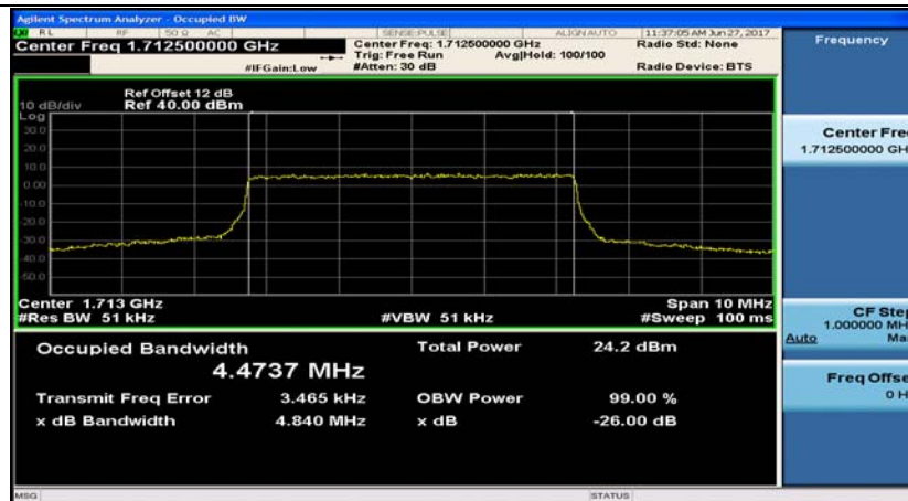
Band4_5MHz_16QAM_19975_25RB#0
