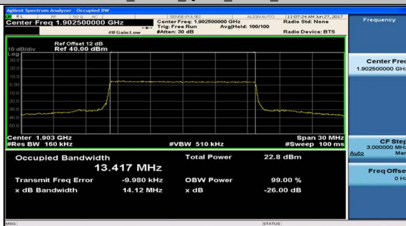
Band2_15MHz_16QAM_19125_75RB#0
