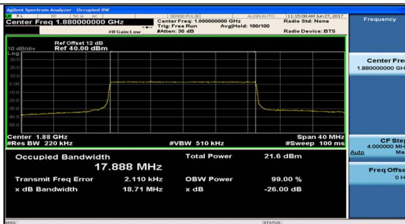
Band2_20MHz_QPSK_19100_100RB#0
