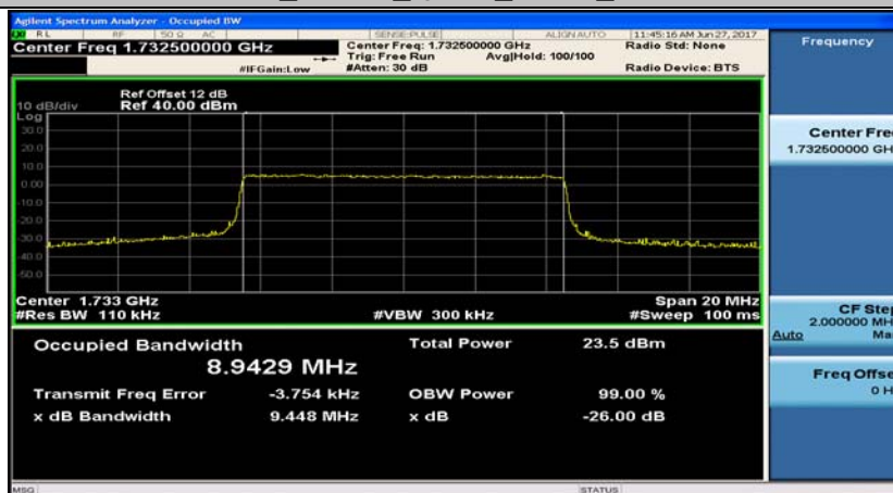
Band4_10MHz_16QAM_20175_50RB#0
