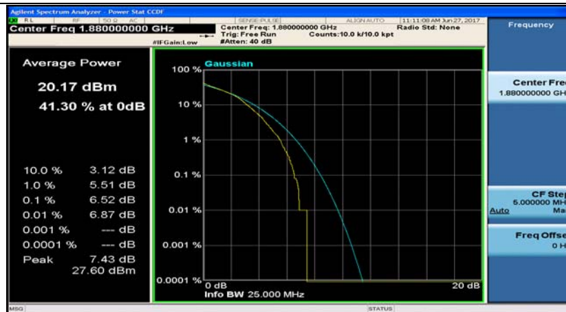
Band2_20MHz_QPSK_18900_100RB#0
