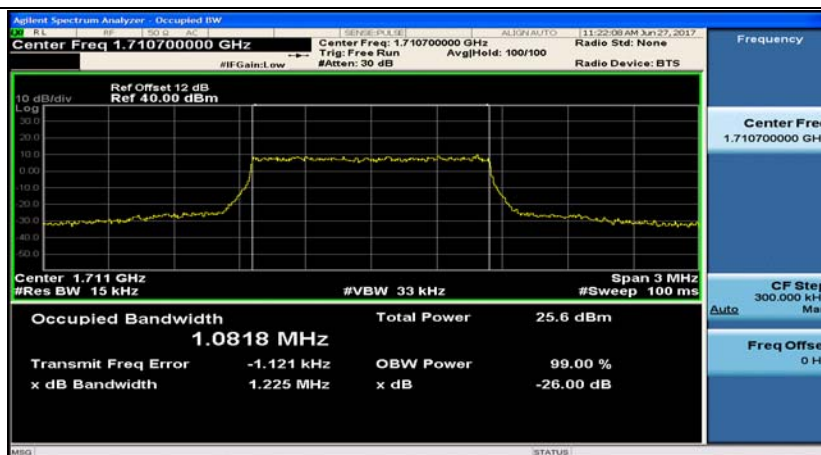
Band4_1.4MHz_16QAM_19957_6RB#0
