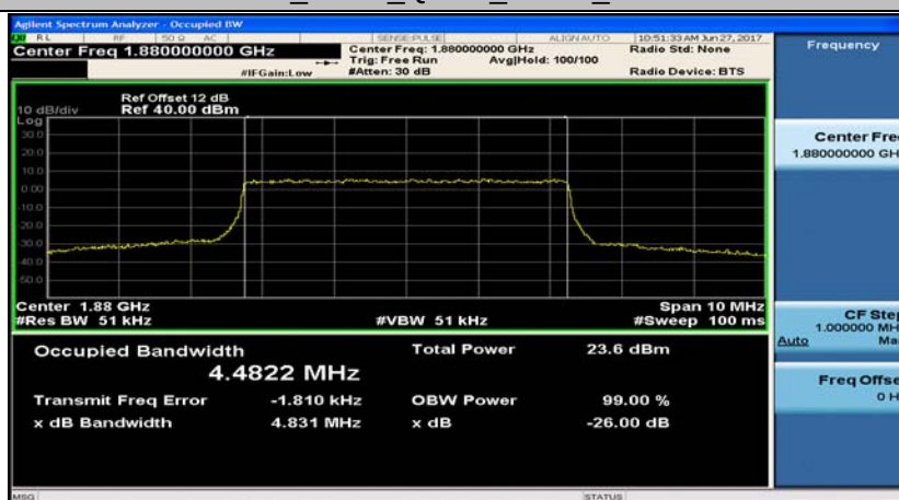
Band2_5MHz_16QAM_18900_25RB#0
