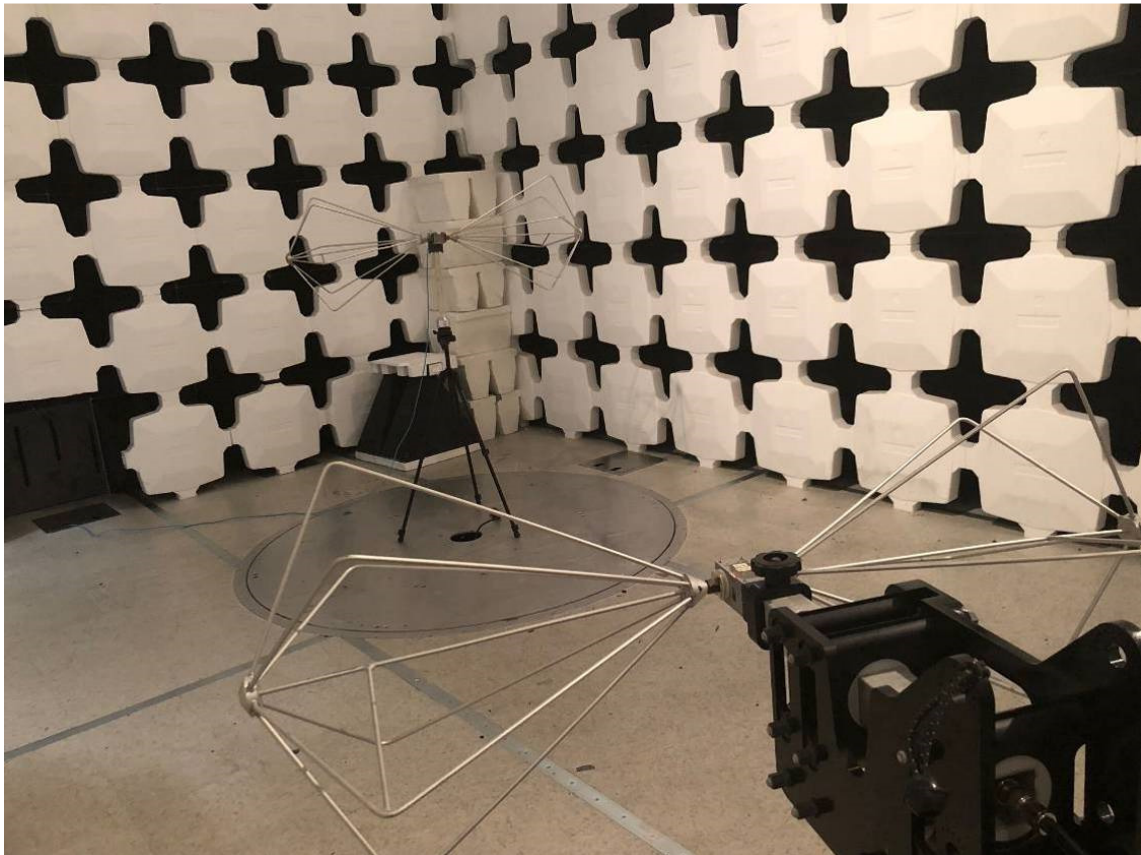
Figure 15. Substitution Testing 30-200 MHz
